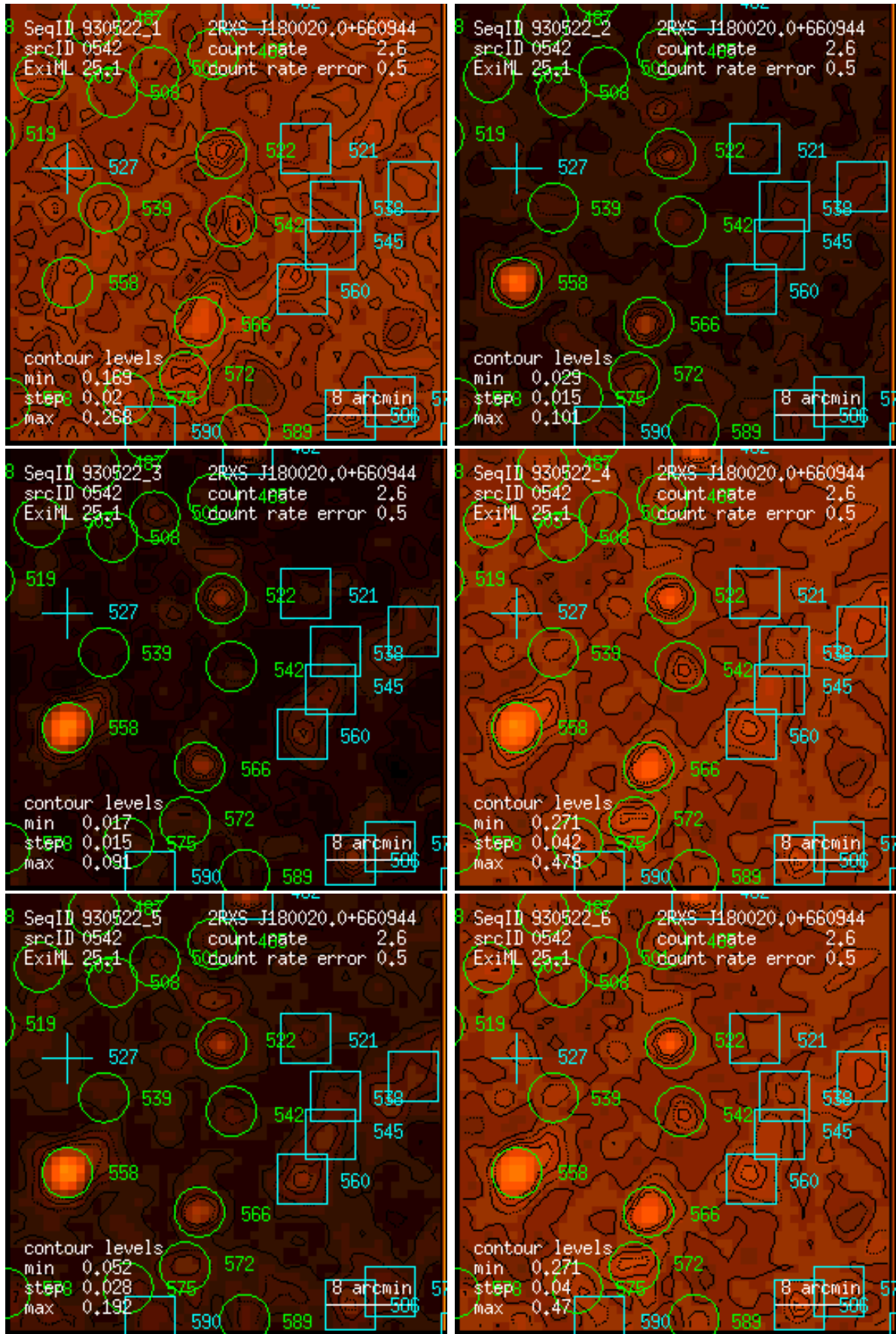
Figure 542: RASS 930522: detection 0542: band rate images, Gaussian filter: (1) PSPC channels 11 – 41, (2) 52 – 90, (3) 91 – 201, (4) 11 – 235, (5) 52 – 201, (6) 11 – 201. Broad band rates in counts/ks. Band rate contour levels in counts/ks/arcmin 2 .
