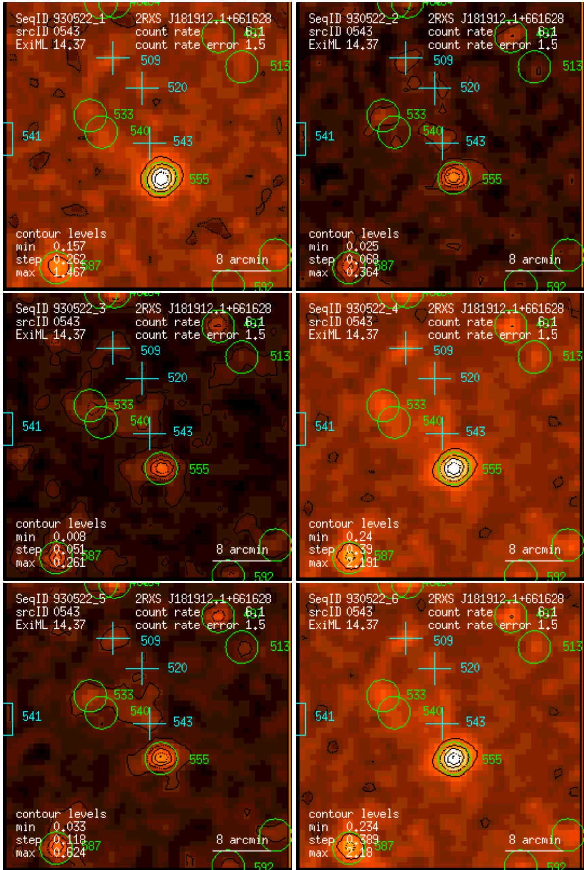
Figure 543: RASS 930522: detection 0543: band rate images, Gaussian filter: (1) PSPC channels 11 – 41, (2) 52 – 90, (3) 91 – 201, (4) 11 – 235, (5) 52 – 201, (6) 11 – 201. Broad band rates in counts/ks. Band rate contour levels in counts/ks/arcmin 2 .
