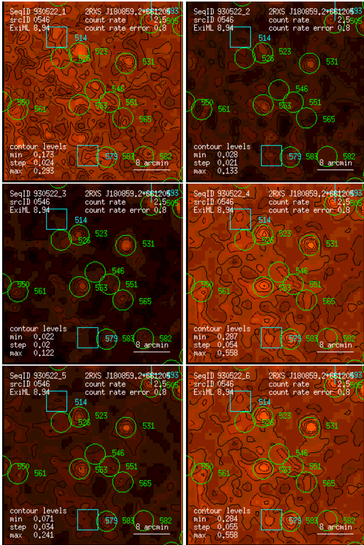
Figure 546: RASS 930522: detection 0546: band rate images, Gaussian filter: (1) PSPC channels 11 – 41, (2) 52 – 90, (3) 91 – 201, (4) 11 – 235, (5) 52 – 201, (6) 11 – 201. Broad band rates in counts/ks. Band rate contour levels in counts/ks/arcmin 2 .
