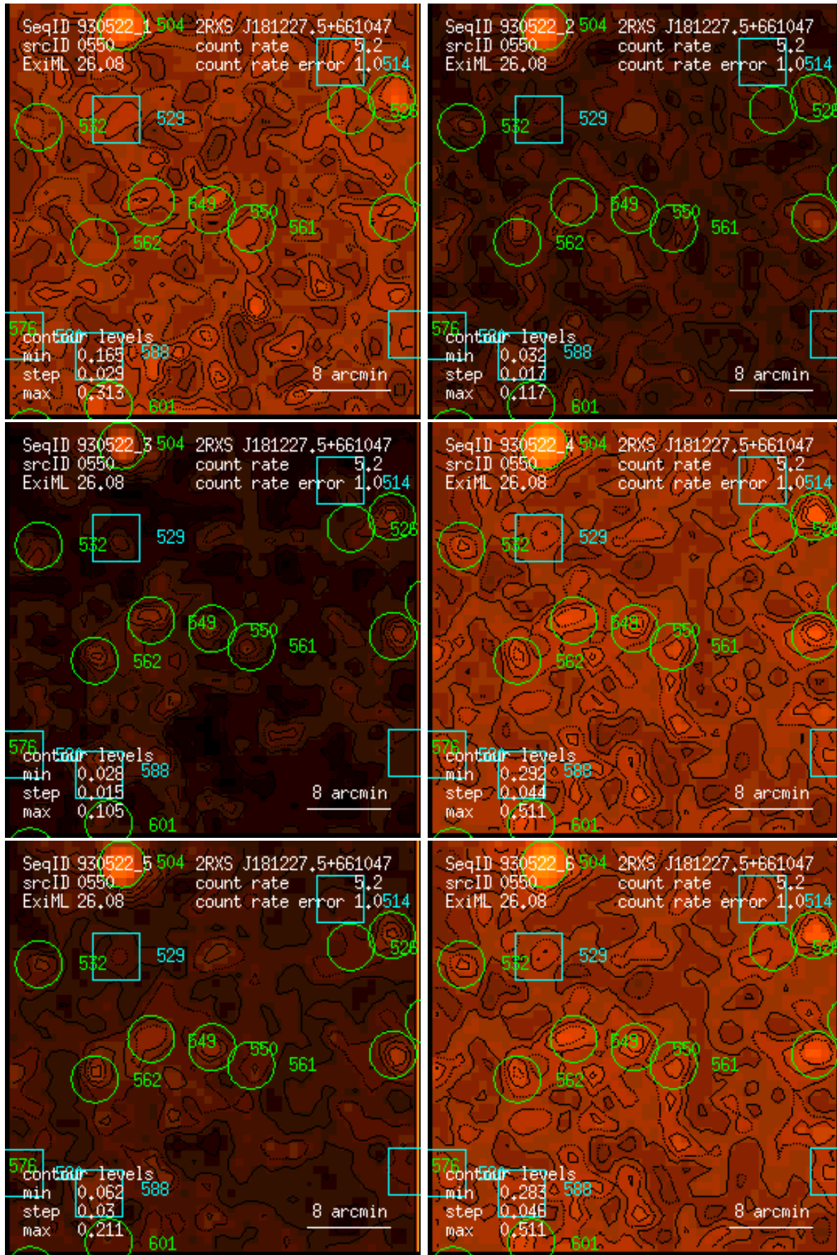
Figure 550: RASS 930522: detection 0550: band rate images, Gaussian filter: (1) PSPC channels 11 – 41, (2) 52 – 90, (3) 91 – 201, (4) 11 – 235, (5) 52 – 201, (6) 11 – 201. Broad band rates in counts/ks. Band rate contour levels in counts/ks/arcmin 2 .
