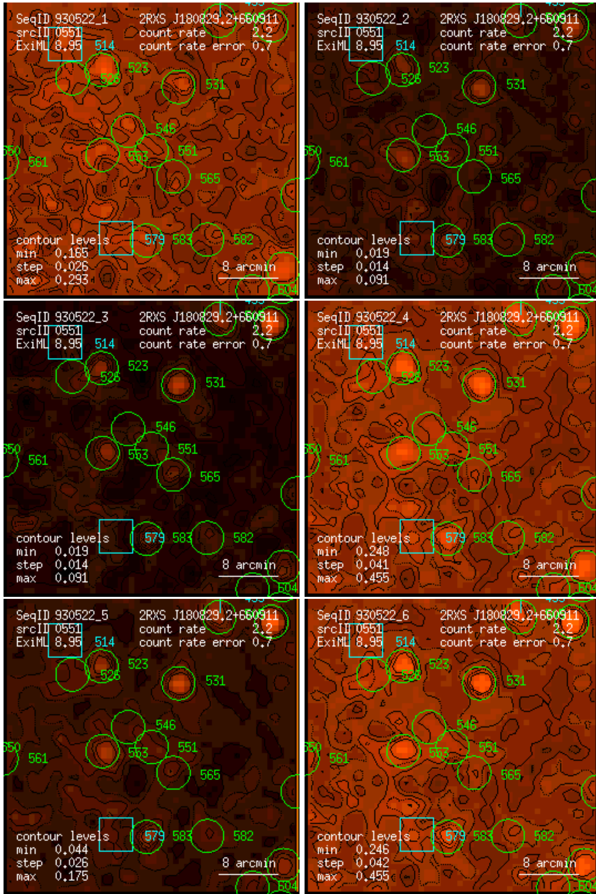
Figure 551: RASS 930522: detection 0551: band rate images, Gaussian filter: (1) PSPC channels 11 – 41, (2) 52 – 90, (3) 91 – 201, (4) 11 – 235, (5) 52 – 201, (6) 11 – 201. Broad band rates in counts/ks. Band rate contour levels in counts/ks/arcmin 2 .
