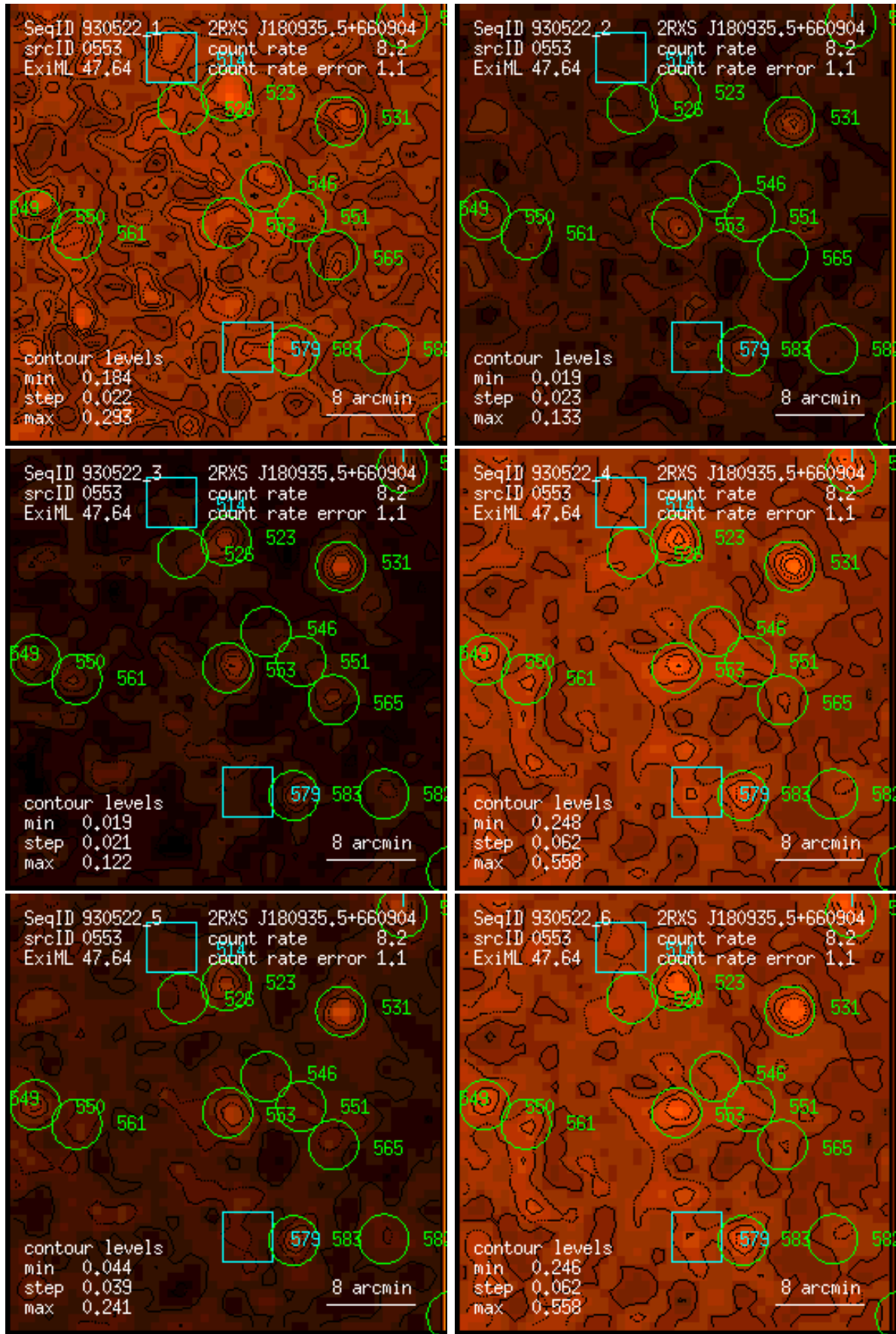
Figure 553: RASS 930522: detection 0553: band rate images, Gaussian filter: (1) PSPC channels 11 – 41, (2) 52 – 90, (3) 91 – 201, (4) 11 – 235, (5) 52 – 201, (6) 11 – 201. Broad band rates in counts/ks. Band rate contour levels in counts/ks/arcmin 2 .
