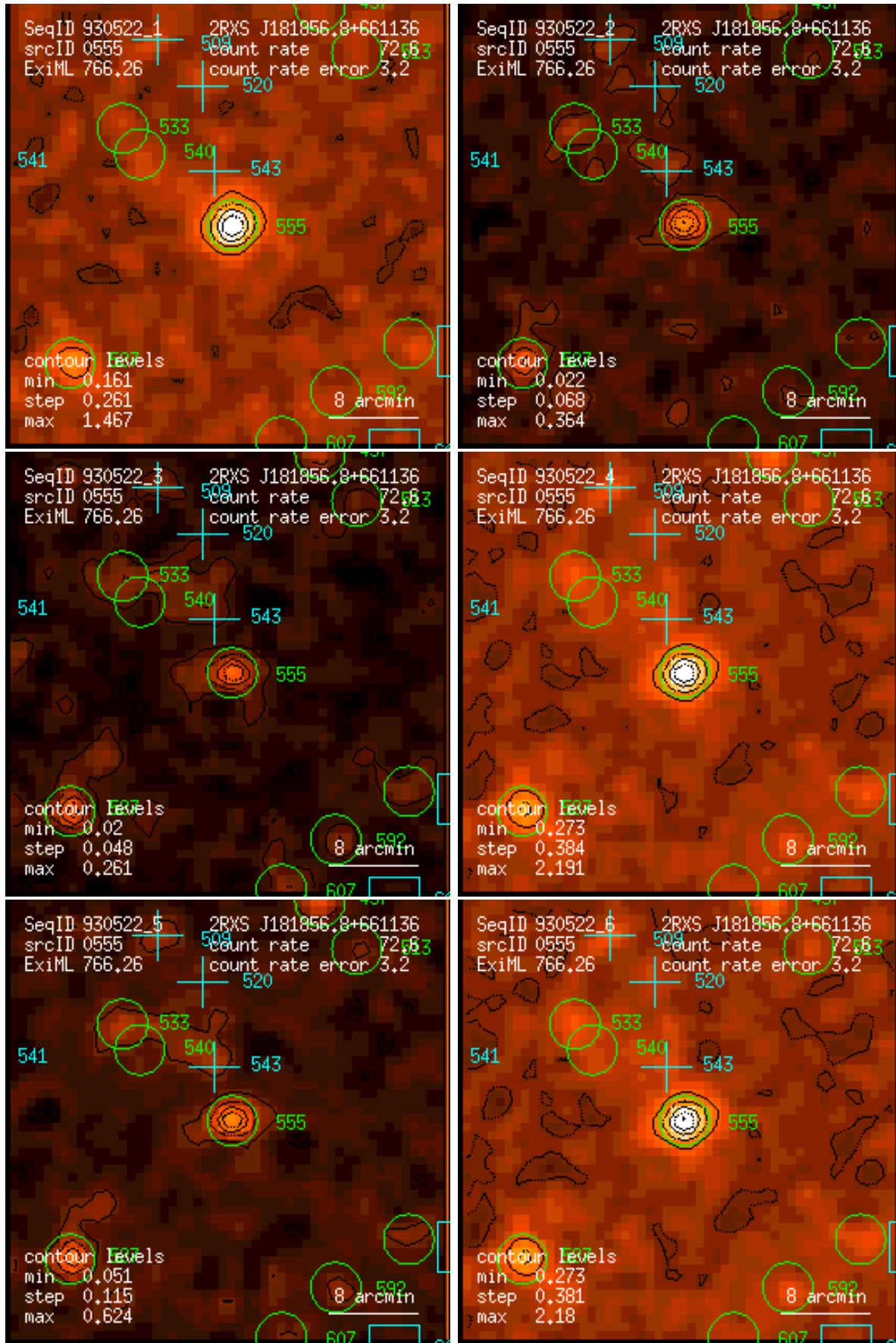
Figure 555: RASS 930522: detection 0555: band rate images, Gaussian filter: (1) PSPC channels 11 – 41, (2) 52 – 90, (3) 91 – 201, (4) 11 – 235, (5) 52 – 201, (6) 11 – 201. Broad band rates in counts/ks. Band rate contour levels in counts/ks/arcmin 2 .
