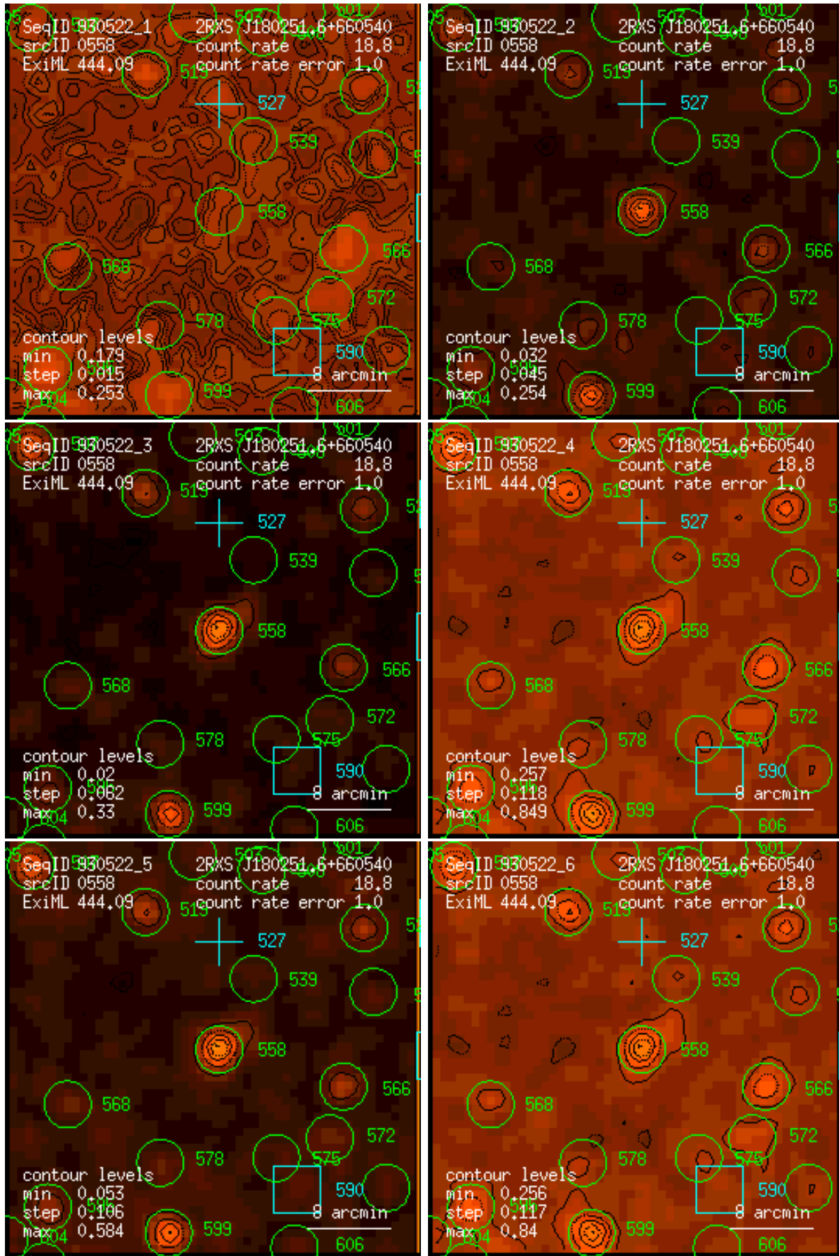
Figure 558: RASS 930522: detection 0558: band rate images, Gaussian filter: (1) PSPC channels 11 – 41, (2) 52 – 90, (3) 91 – 201, (4) 11 – 235, (5) 52 – 201, (6) 11 – 201. Broad band rates in counts/ks. Band rate contour levels in counts/ks/arcmin 2 .
