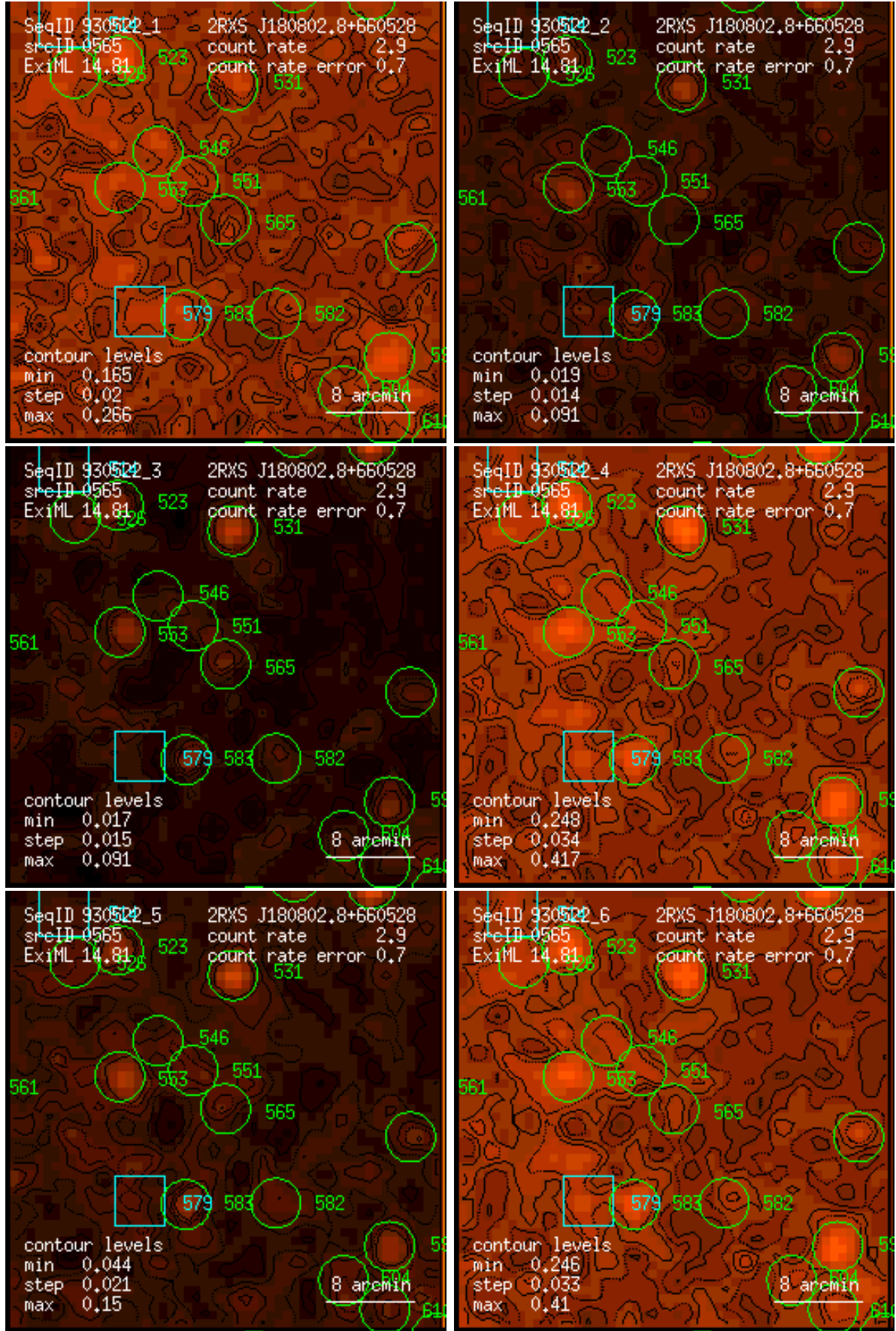
Figure 565: RASS 930522: detection 0565: band rate images, Gaussian filter: (1) PSPC channels 11 – 41, (2) 52 – 90, (3) 91 – 201, (4) 11 – 235, (5) 52 – 201, (6) 11 – 201. Broad band rates in counts/ks. Band rate contour levels in counts/ks/arcmin 2 .
