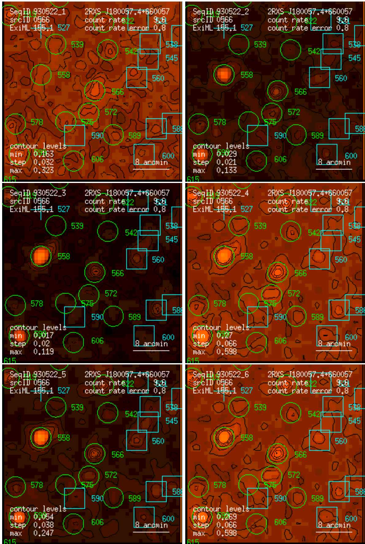
Figure 566: RASS 930522: detection 0566: band rate images, Gaussian filter: (1) PSPC channels 11 – 41, (2) 52 – 90, (3) 91 – 201, (4) 11 – 235, (5) 52 – 201, (6) 11 – 201. Broad band rates in counts/ks. Band rate contour levels in counts/ks/arcmin 2 .
