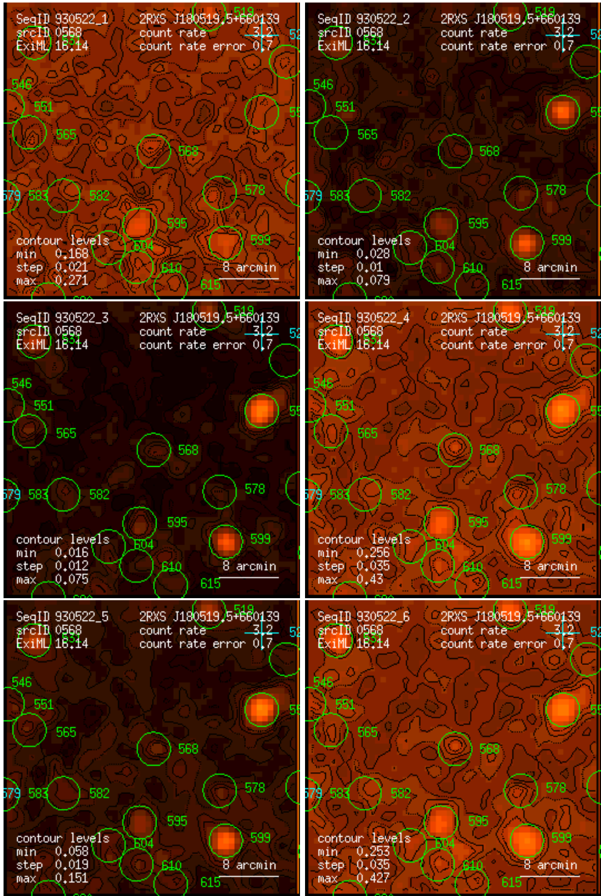
Figure 568: RASS 930522: detection 0568: band rate images, Gaussian filter: (1) PSPC channels 11 – 41, (2) 52 – 90, (3) 91 – 201, (4) 11 – 235, (5) 52 – 201, (6) 11 – 201. Broad band rates in counts/ks. Band rate contour levels in counts/ks/arcmin 2 .
