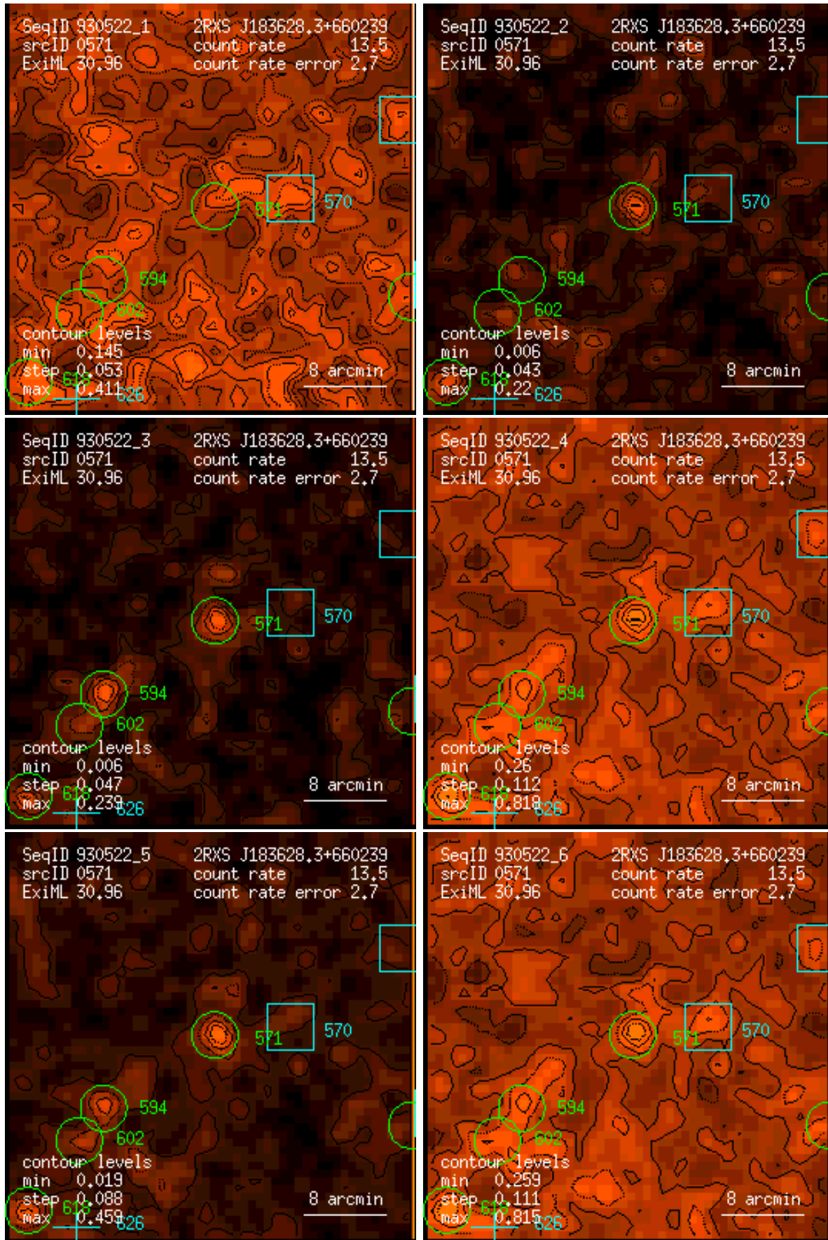
Figure 571: RASS 930522: detection 0571: band rate images, Gaussian filter: (1) PSPC channels 11 – 41, (2) 52 – 90, (3) 91 – 201, (4) 11 – 235, (5) 52 – 201, (6) 11 – 201. Broad band rates in counts/ks. Band rate contour levels in counts/ks/arcmin 2 .
