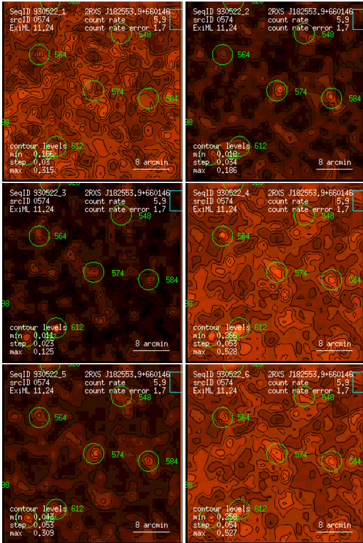
Figure 574: RASS 930522: detection 0574: band rate images, Gaussian filter: (1) PSPC channels 11 – 41, (2) 52 – 90, (3) 91 – 201, (4) 11 – 235, (5) 52 – 201, (6) 11 – 201. Broad band rates in counts/ks. Band rate contour levels in counts/ks/arcmin 2 .
