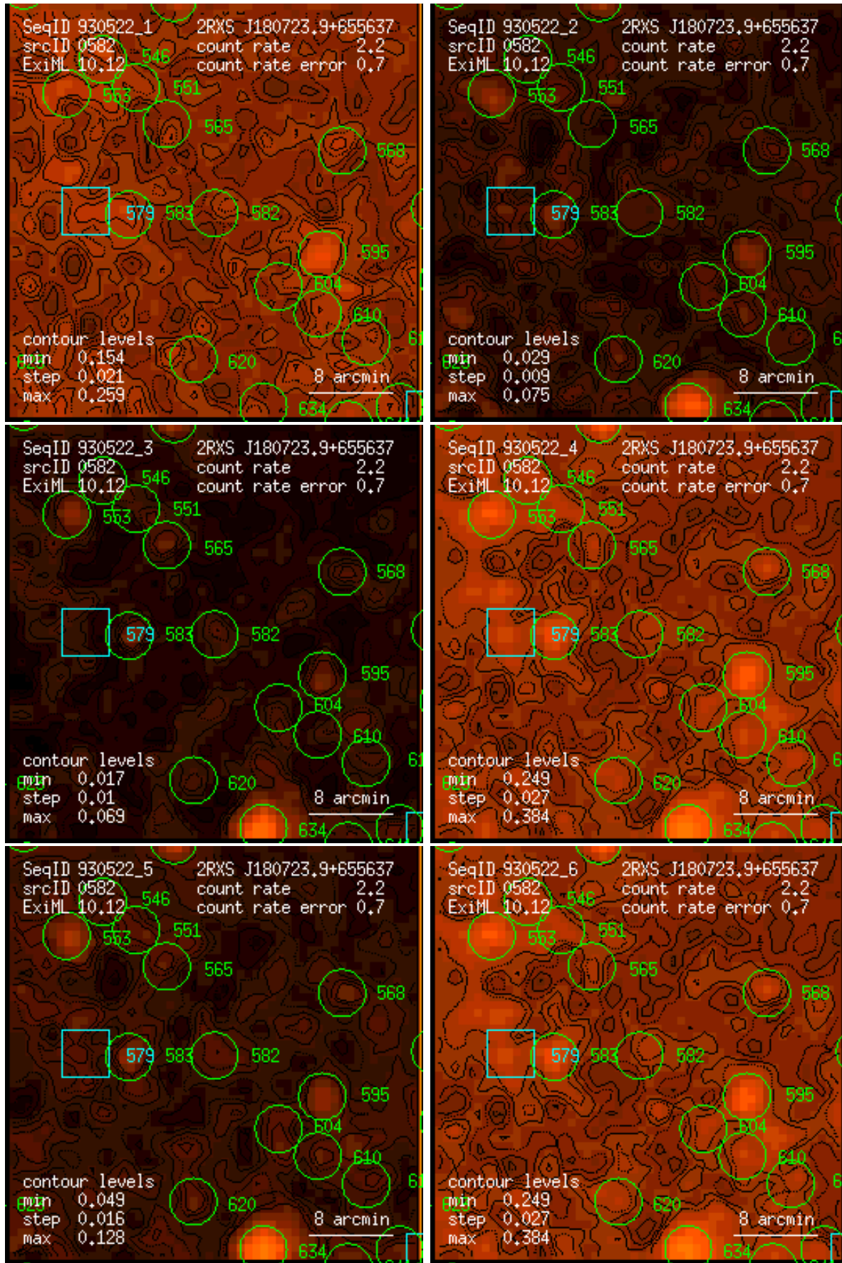
Figure 582: RASS 930522: detection 0582: band rate images, Gaussian filter: (1) PSPC channels 11 – 41, (2) 52 – 90, (3) 91 – 201, (4) 11 – 235, (5) 52 – 201, (6) 11 – 201. Broad band rates in counts/ks. Band rate contour levels in counts/ks/arcmin 2 .
