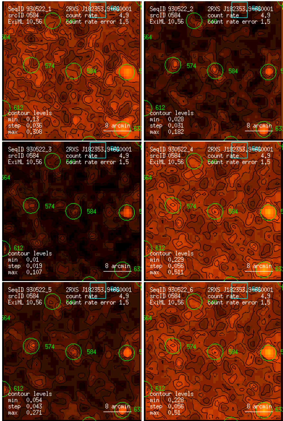
Figure 584: RASS 930522: detection 0584: band rate images, Gaussian filter: (1) PSPC channels 11 – 41, (2) 52 – 90, (3) 91 – 201, (4) 11 – 235, (5) 52 – 201, (6) 11 – 201. Broad band rates in counts/ks. Band rate contour levels in counts/ks/arcmin 2 .
