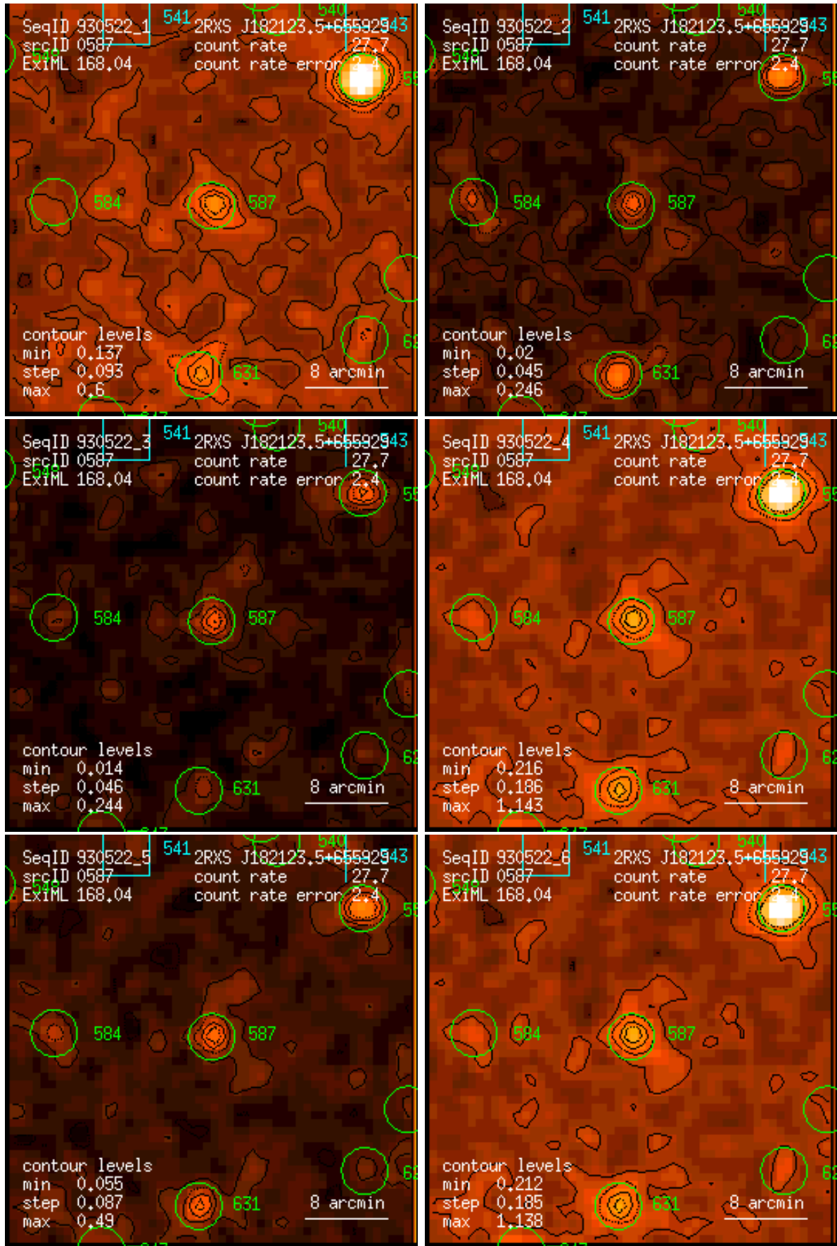
Figure 587: RASS 930522: detection 0587: band rate images, Gaussian filter: (1) PSPC channels 11 – 41, (2) 52 – 90, (3) 91 – 201, (4) 11 – 235, (5) 52 – 201, (6) 11 – 201. Broad band rates in counts/ks. Band rate contour levels in counts/ks/arcmin 2 .
