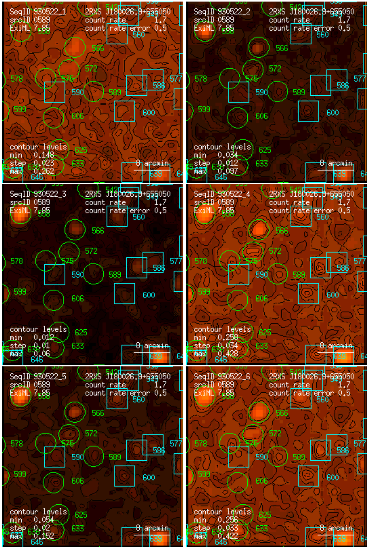
Figure 589: RASS 930522: detection 0589: band rate images, Gaussian filter: (1) PSPC channels 11 – 41, (2) 52 – 90, (3) 91 – 201, (4) 11 – 235, (5) 52 – 201, (6) 11 – 201. Broad band rates in counts/ks. Band rate contour levels in counts/ks/arcmin 2 .
