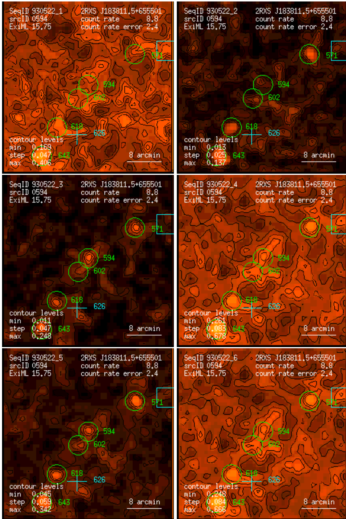
Figure 594: RASS 930522: detection 0594: band rate images, Gaussian filter: (1) PSPC channels 11 – 41, (2) 52 – 90, (3) 91 – 201, (4) 11 – 235, (5) 52 – 201, (6) 11 – 201. Broad band rates in counts/ks. Band rate contour levels in counts/ks/arcmin 2 .
