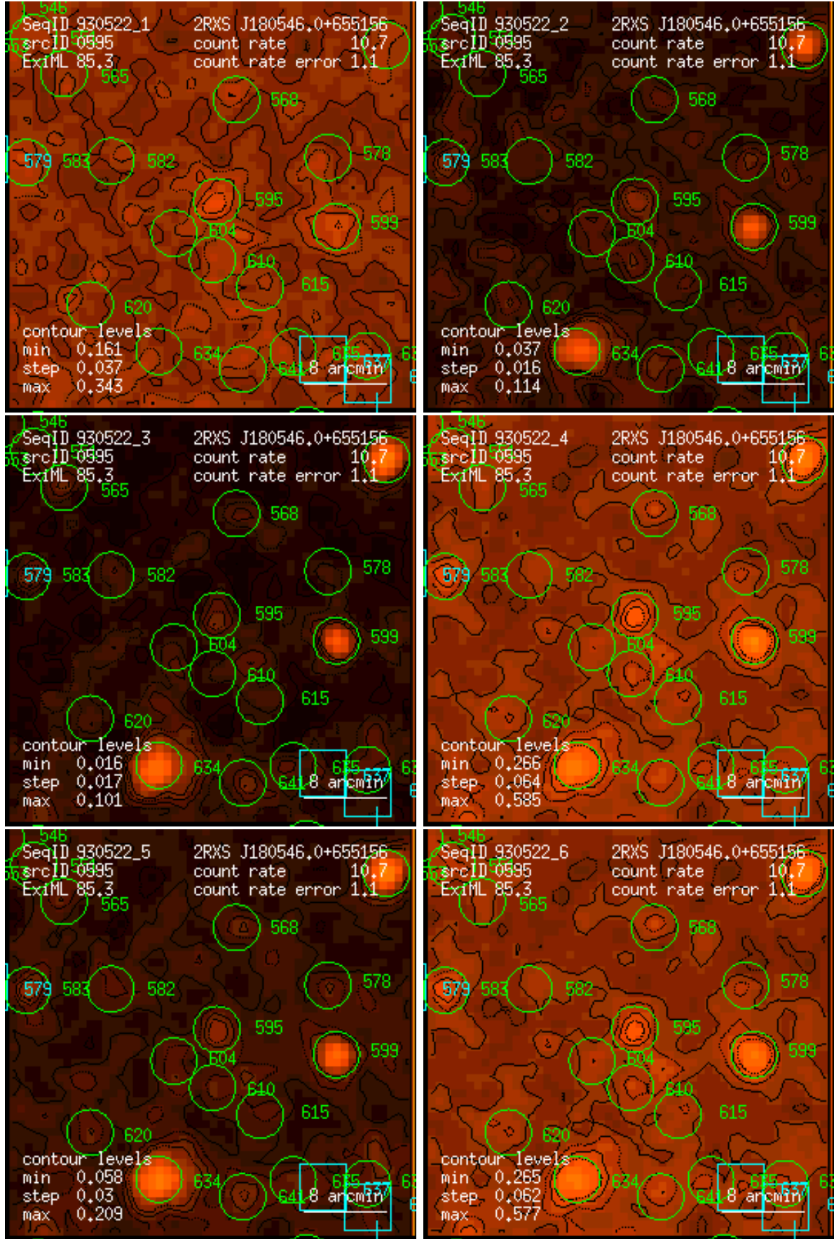
Figure 595: RASS 930522: detection 0595: band rate images, Gaussian filter: (1) PSPC channels 11 – 41, (2) 52 – 90, (3) 91 – 201, (4) 11 – 235, (5) 52 – 201, (6) 11 – 201. Broad band rates in counts/ks. Band rate contour levels in counts/ks/arcmin 2 .
