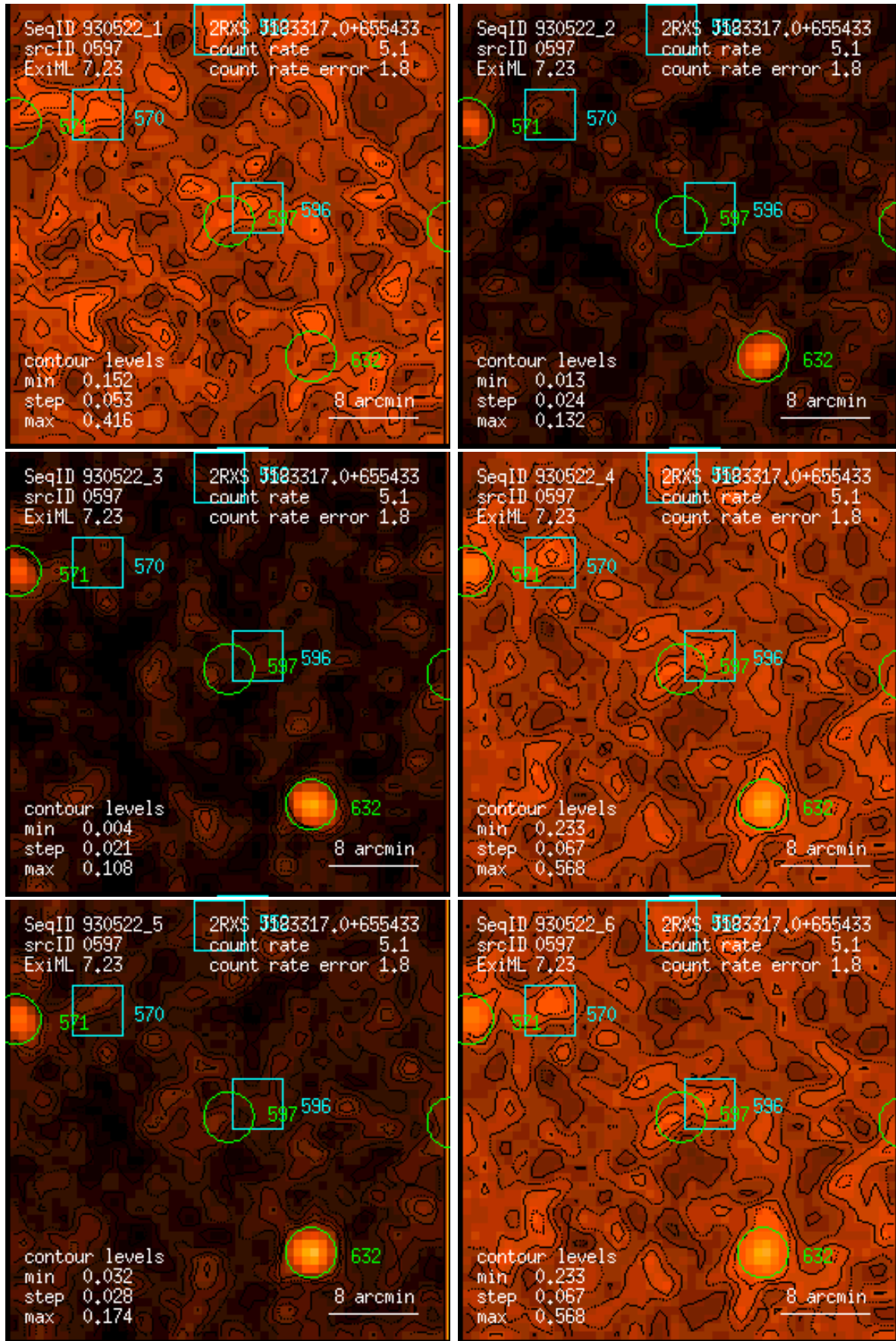
Figure 597: RASS 930522: detection 0597: band rate images, Gaussian filter: (1) PSPC channels 11 – 41, (2) 52 – 90, (3) 91 – 201, (4) 11 – 235, (5) 52 – 201, (6) 11 – 201. Broad band rates in counts/ks. Band rate contour levels in counts/ks/arcmin 2 .
