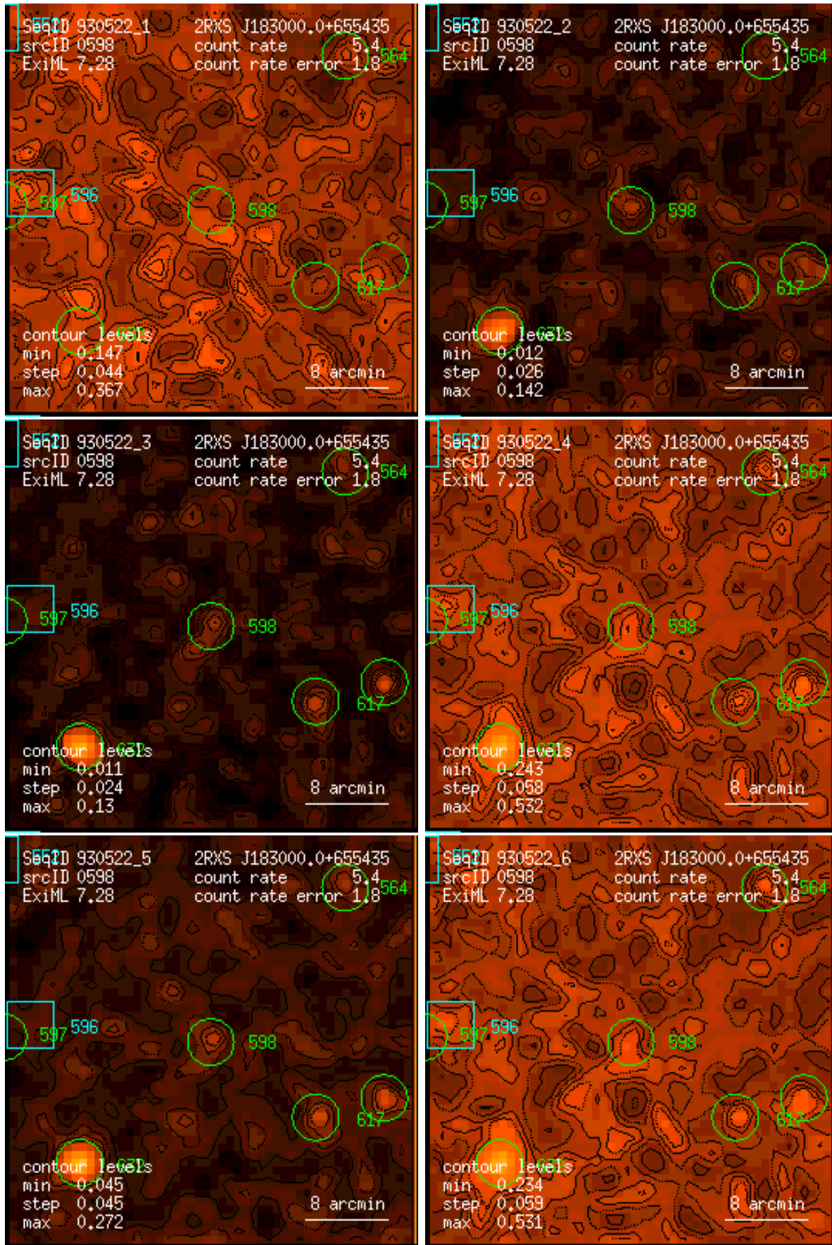
Figure 598: RASS 930522: detection 0598: band rate images, Gaussian filter: (1) PSPC channels 11 – 41, (2) 52 – 90, (3) 91 – 201, (4) 11 – 235, (5) 52 – 201, (6) 11 – 201. Broad band rates in counts/ks. Band rate contour levels in counts/ks/arcmin 2 .
