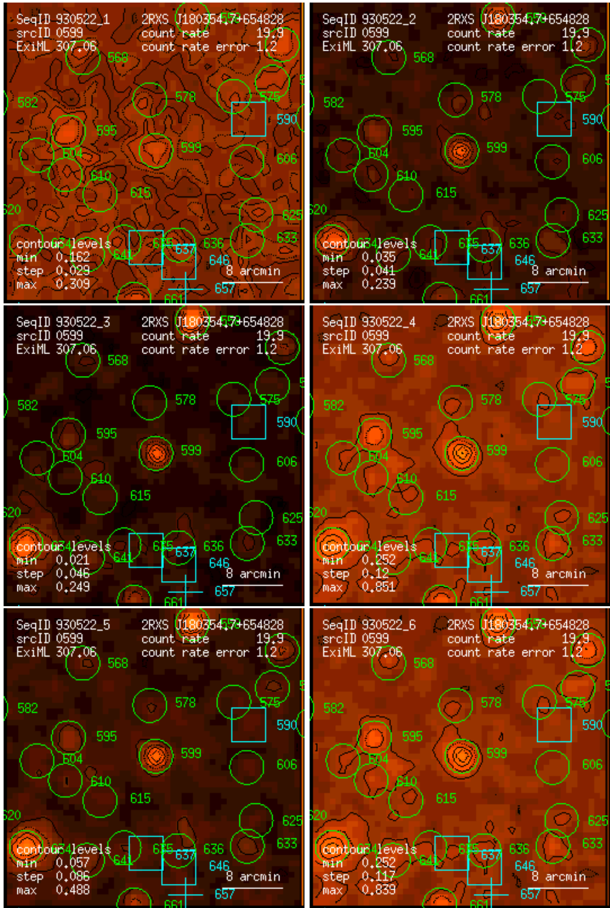
Figure 599: RASS 930522: detection 0599: band rate images, Gaussian filter: (1) PSPC channels 11 – 41, (2) 52 – 90, (3) 91 – 201, (4) 11 – 235, (5) 52 – 201, (6) 11 – 201. Broad band rates in counts/ks. Band rate contour levels in counts/ks/arcmin 2 .
