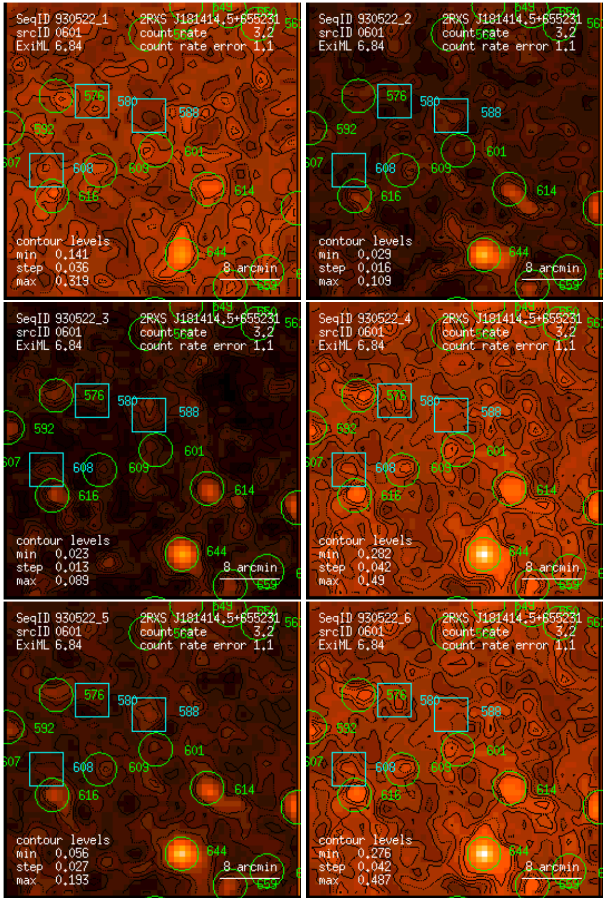
Figure 601: RASS 930522: detection 0601: band rate images, Gaussian filter: (1) PSPC channels 11 – 41, (2) 52 – 90, (3) 91 – 201, (4) 11 – 235, (5) 52 – 201, (6) 11 – 201. Broad band rates in counts/ks. Band rate contour levels in counts/ks/arcmin 2 .
