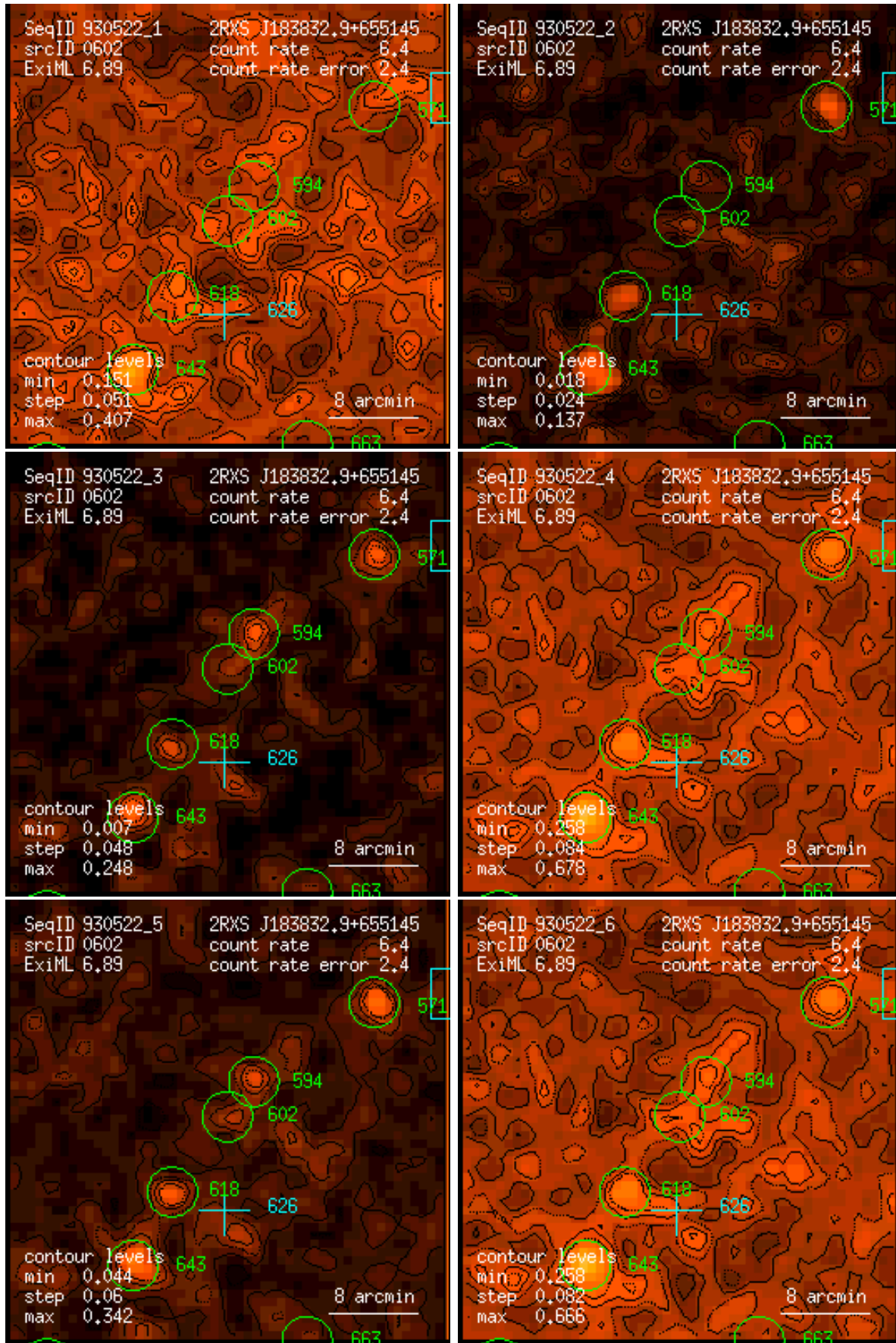
Figure 602: RASS 930522: detection 0602: band rate images, Gaussian filter: (1) PSPC channels 11 – 41, (2) 52 – 90, (3) 91 – 201, (4) 11 – 235, (5) 52 – 201, (6) 11 – 201. Broad band rates in counts/ks. Band rate contour levels in counts/ks/arcmin 2 .
