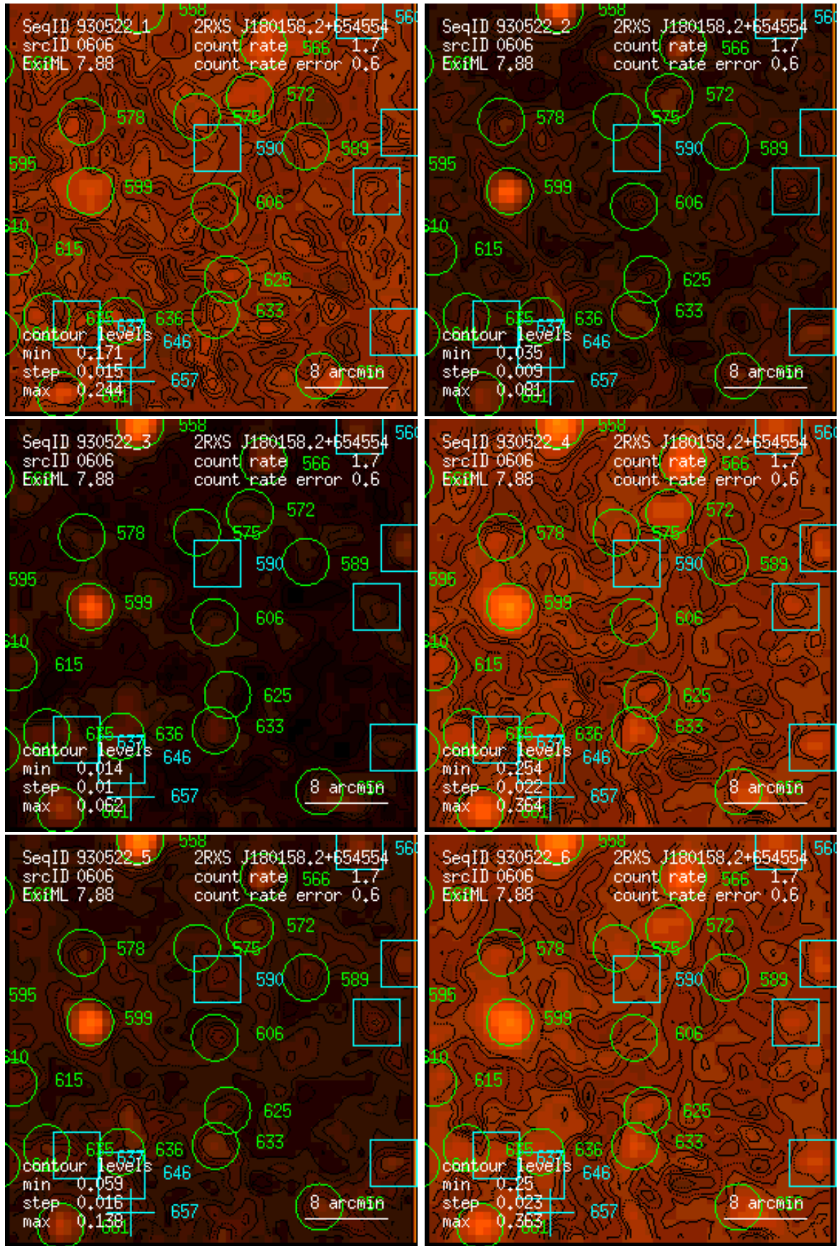
Figure 606: RASS 930522: detection 0606: band rate images, Gaussian filter: (1) PSPC channels 11 – 41, (2) 52 – 90, (3) 91 – 201, (4) 11 – 235, (5) 52 – 201, (6) 11 – 201. Broad band rates in counts/ks. Band rate contour levels in counts/ks/arcmin 2 .
