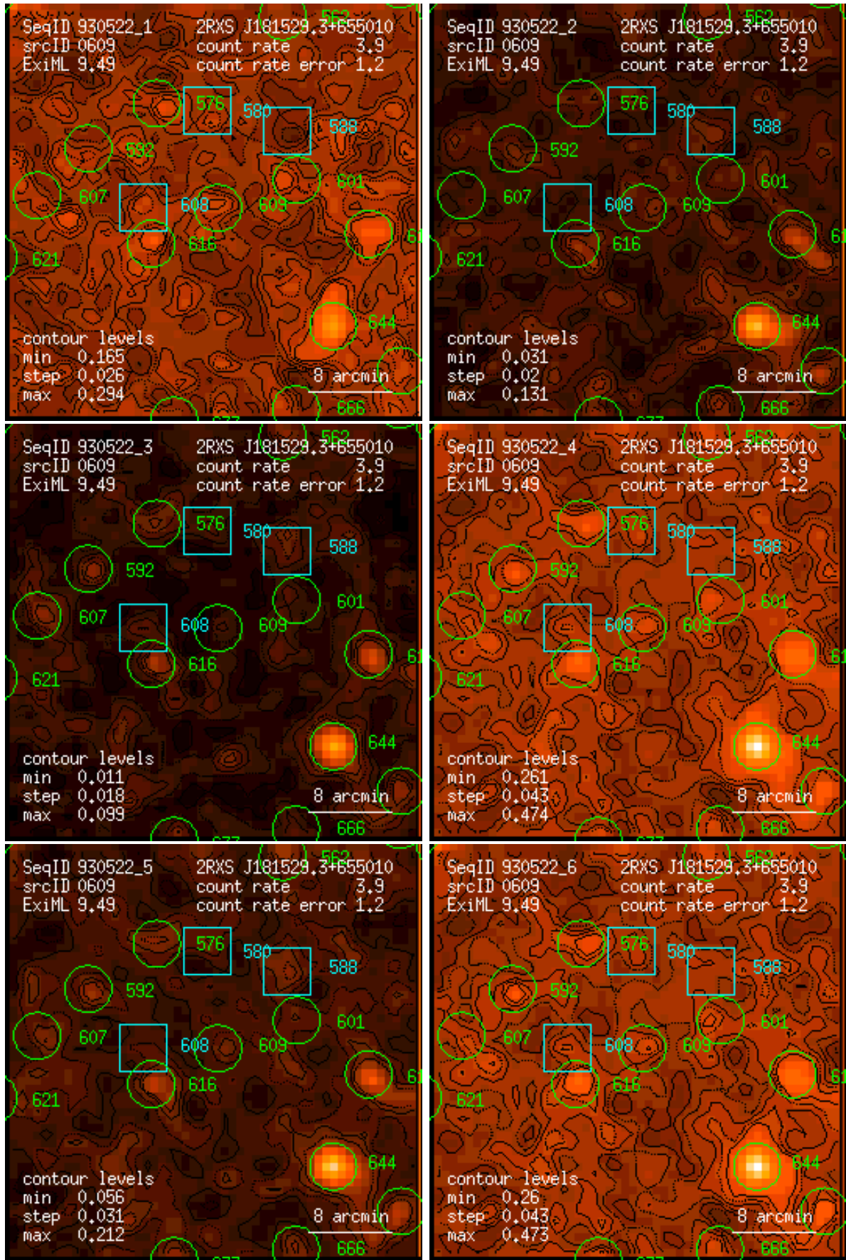
Figure 609: RASS 930522: detection 0609: band rate images, Gaussian filter: (1) PSPC channels 11 – 41, (2) 52 – 90, (3) 91 – 201, (4) 11 – 235, (5) 52 – 201, (6) 11 – 201. Broad band rates in counts/ks. Band rate contour levels in counts/ks/arcmin 2 .
