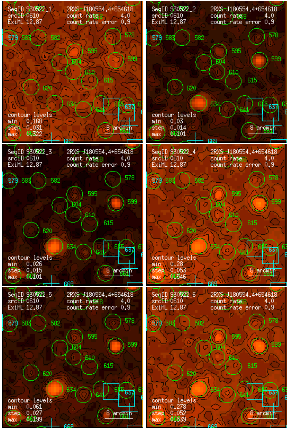
Figure 610: RASS 930522: detection 0610: band rate images, Gaussian filter: (1) PSPC channels 11 – 41, (2) 52 – 90, (3) 91 – 201, (4) 11 – 235, (5) 52 – 201, (6) 11 – 201. Broad band rates in counts/ks. Band rate contour levels in counts/ks/arcmin 2 .
