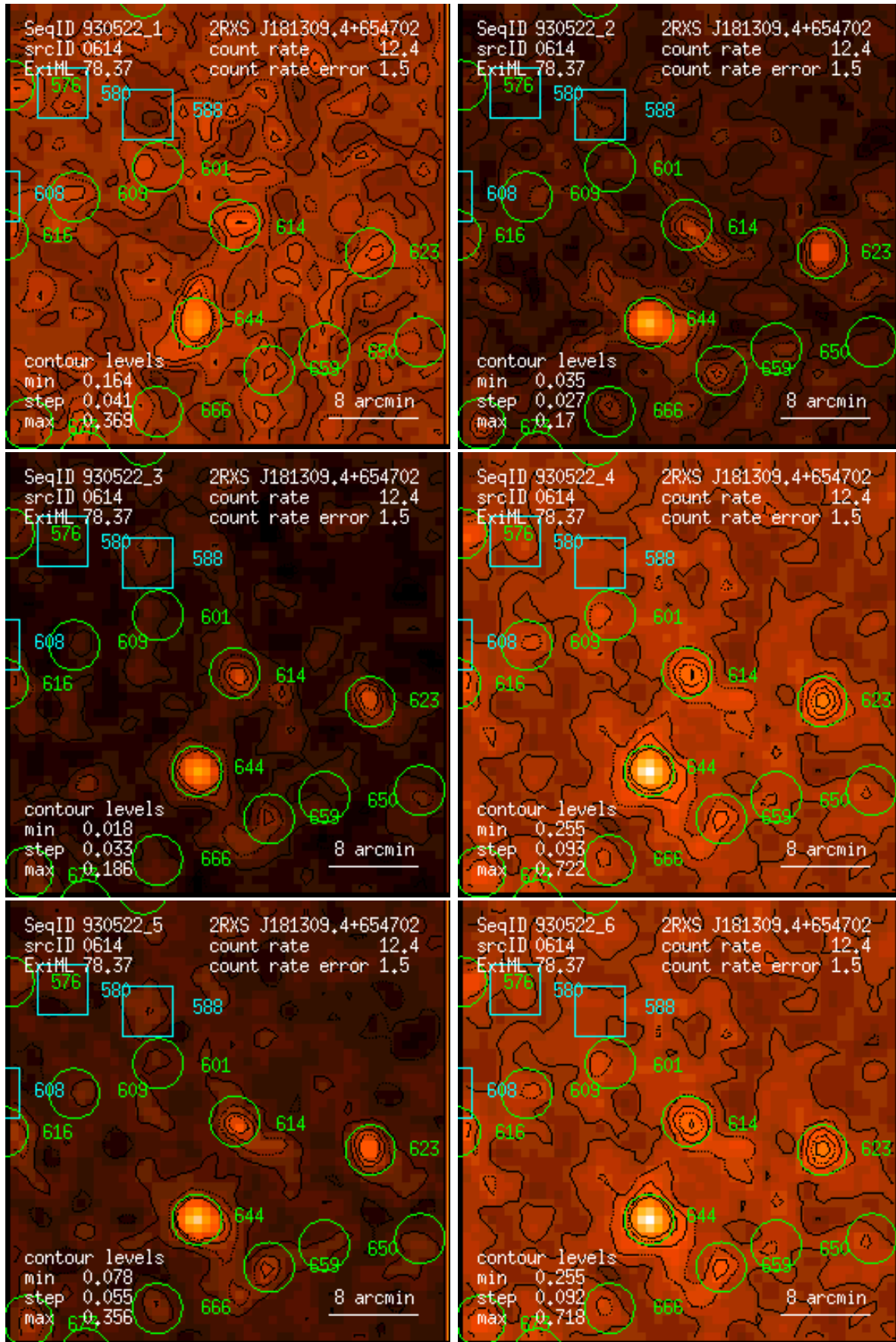
Figure 614: RASS 930522: detection 0614: band rate images, Gaussian filter: (1) PSPC channels 11 – 41, (2) 52 – 90, (3) 91 – 201, (4) 11 – 235, (5) 52 – 201, (6) 11 – 201. Broad band rates in counts/ks. Band rate contour levels in counts/ks/arcmin 2 .
