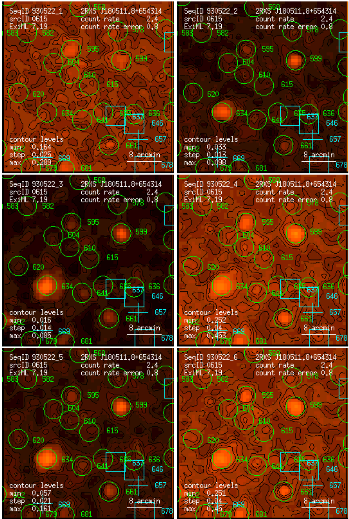
Figure 615: RASS 930522: detection 0615: band rate images, Gaussian filter: (1) PSPC channels 11 – 41, (2) 52 – 90, (3) 91 – 201, (4) 11 – 235, (5) 52 – 201, (6) 11 – 201. Broad band rates in counts/ks. Band rate contour levels in counts/ks/arcmin 2 .
