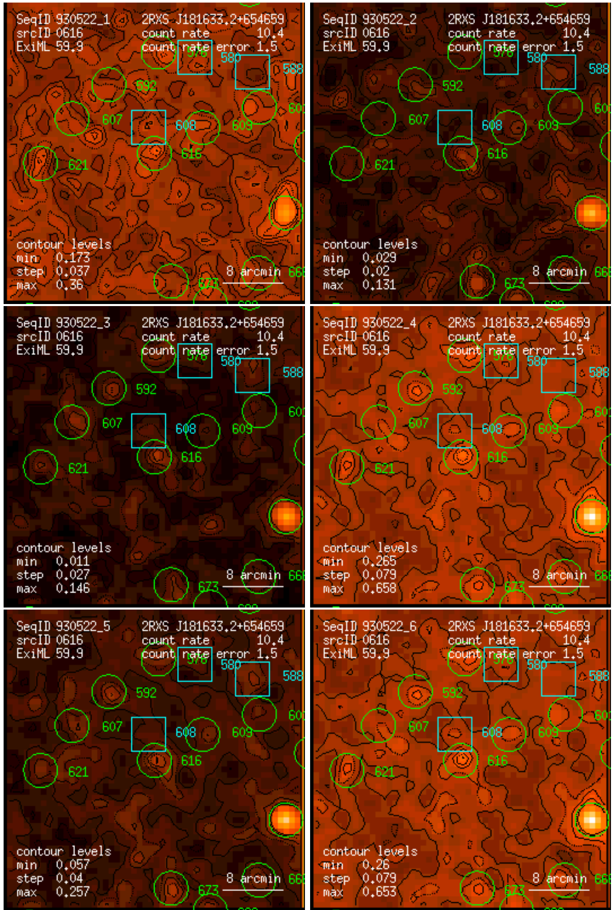
Figure 616: RASS 930522: detection 0616: band rate images, Gaussian filter: (1) PSPPC channels 11 – 41, (2) 52 – 90, (3) 91 – 201, (4) 11 – 235, (5) 52 – 201, (6) 11 – 201. Broad band rates in counts/ks. Band rate contour levels in counts/ks/arcmin 2 .
