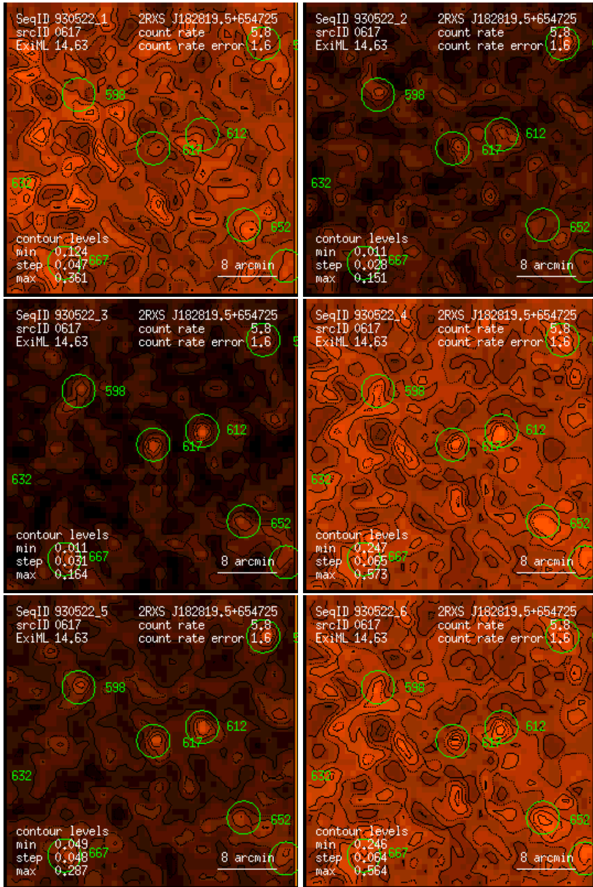
Figure 617: RASS 930522: detection 0617: band rate images, Gaussian filter: (1) PSPC channels 11 – 41, (2) 52 – 90, (3) 91 – 201, (4) 11 – 235, (5) 52 – 201, (6) 11 – 201. Broad band rates in counts/ks. Band rate contour levels in counts/ks/arcmin 2 .
