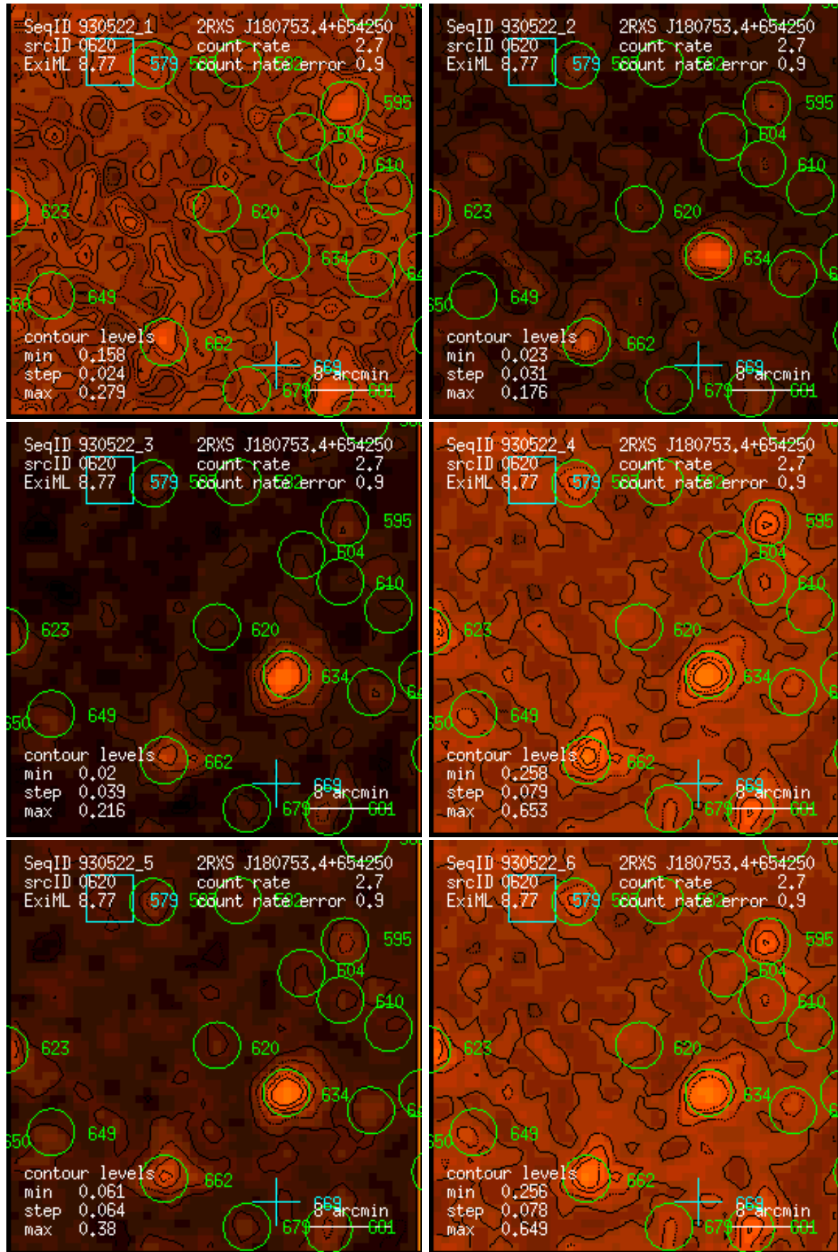
Figure 620: RASS 930522: detection 0620: band rate images, Gaussian filter: (1) PSPC channels 11 – 41, (2) 52 – 90, (3) 91 – 201, (4) 11 – 235, (5) 52 – 201, (6) 11 – 201. Broad band rates in counts/ks. Band rate contour levels in counts/ks/arcmin 2 .
