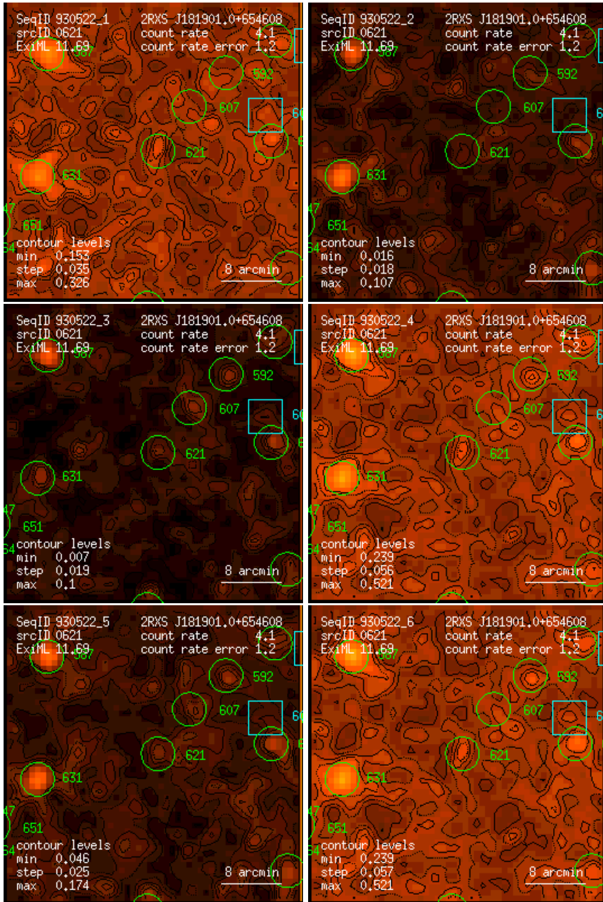
Figure 621: RASS 930522: detection 0621: band rate images, Gaussian filter: (1) PSPC channels 11 – 41, (2) 52 – 90, (3) 91 – 201, (4) 11 – 235, (5) 52 – 201, (6) 11 – 201. Broad band rates in counts/ks. Band rate contour levels in counts/ks/arcmin 2 .
