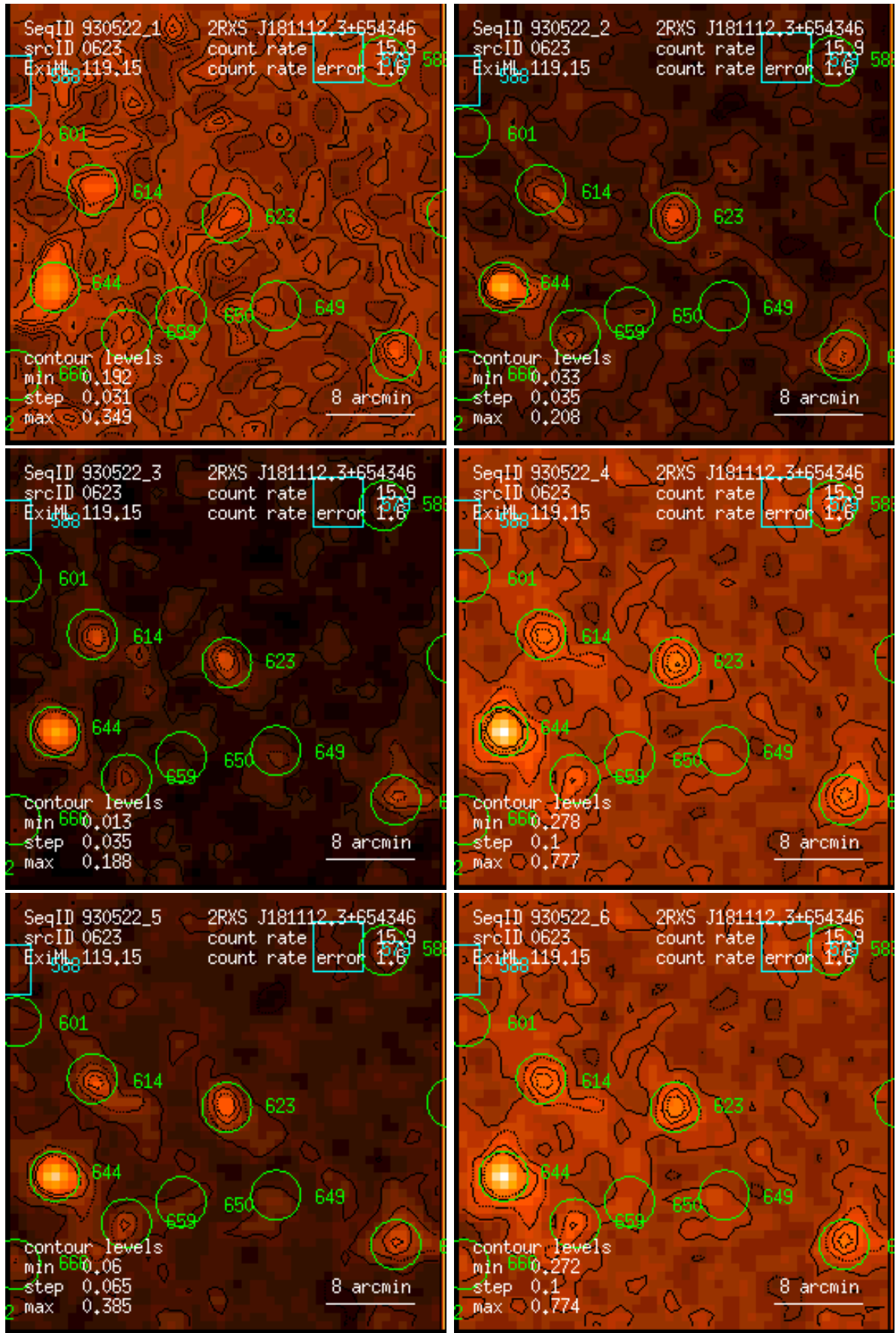
Figure 623: RASS 930522: detection 0623: band rate images, Gaussian filter: (1) PSPC channels 11 – 41, (2) 52 – 90, (3) 91 – 201, (4) 11 – 235, (5) 52 – 201, (6) 11 – 201. Broad band rates in counts/ks. Band rate contour levels in counts/ks/arcmin 2 .
