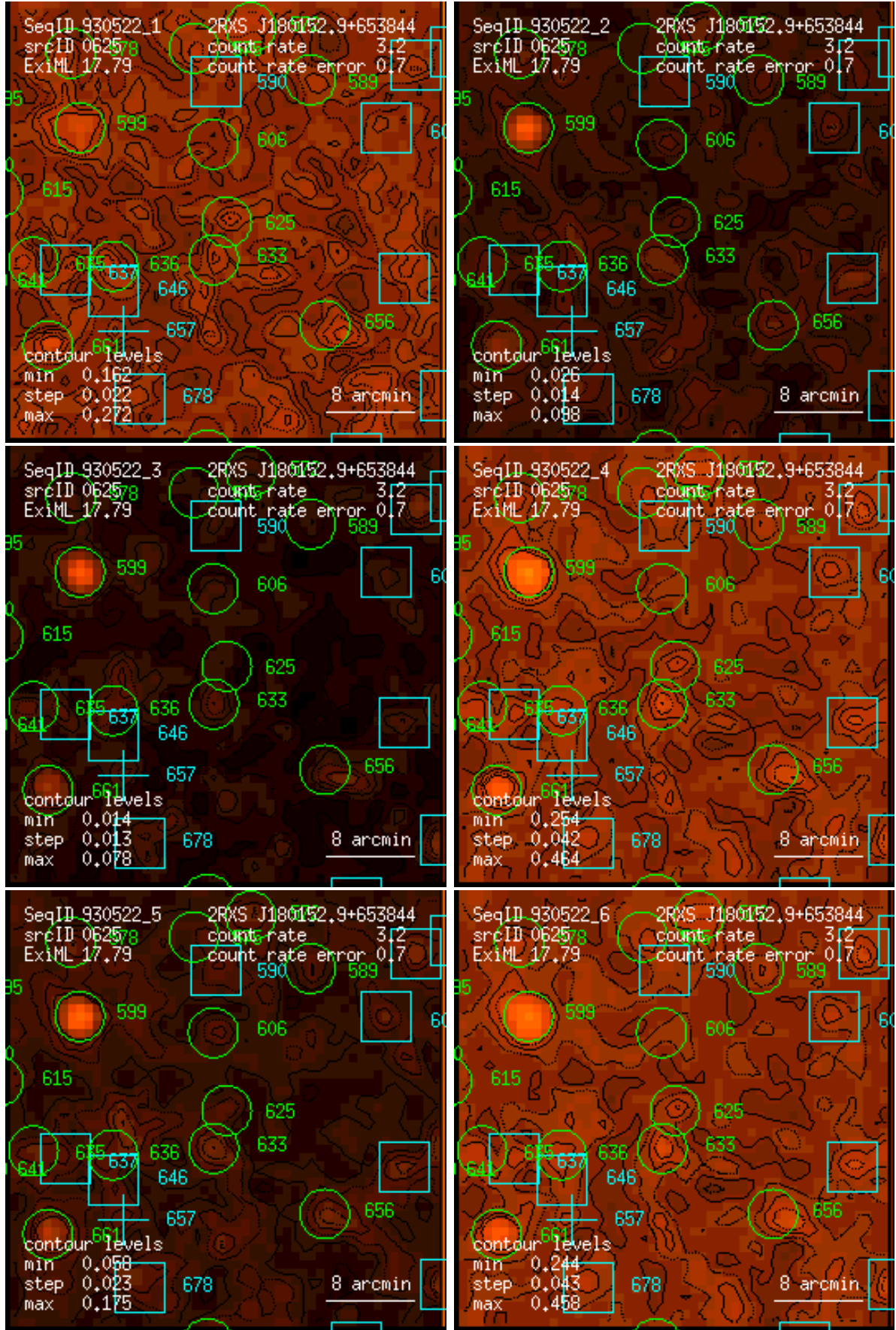
Figure 625: RASS 930522: detection 0625: band rate images, Gaussian filter: (1) PSPC channels 11 – 41, (2) 52 – 90, (3) 91 – 201, (4) 11 – 235, (5) 52 – 201, (6) 11 – 201. Broad band rates in counts/ks. Band rate contour levels in counts/ks/arcmin 2 .
