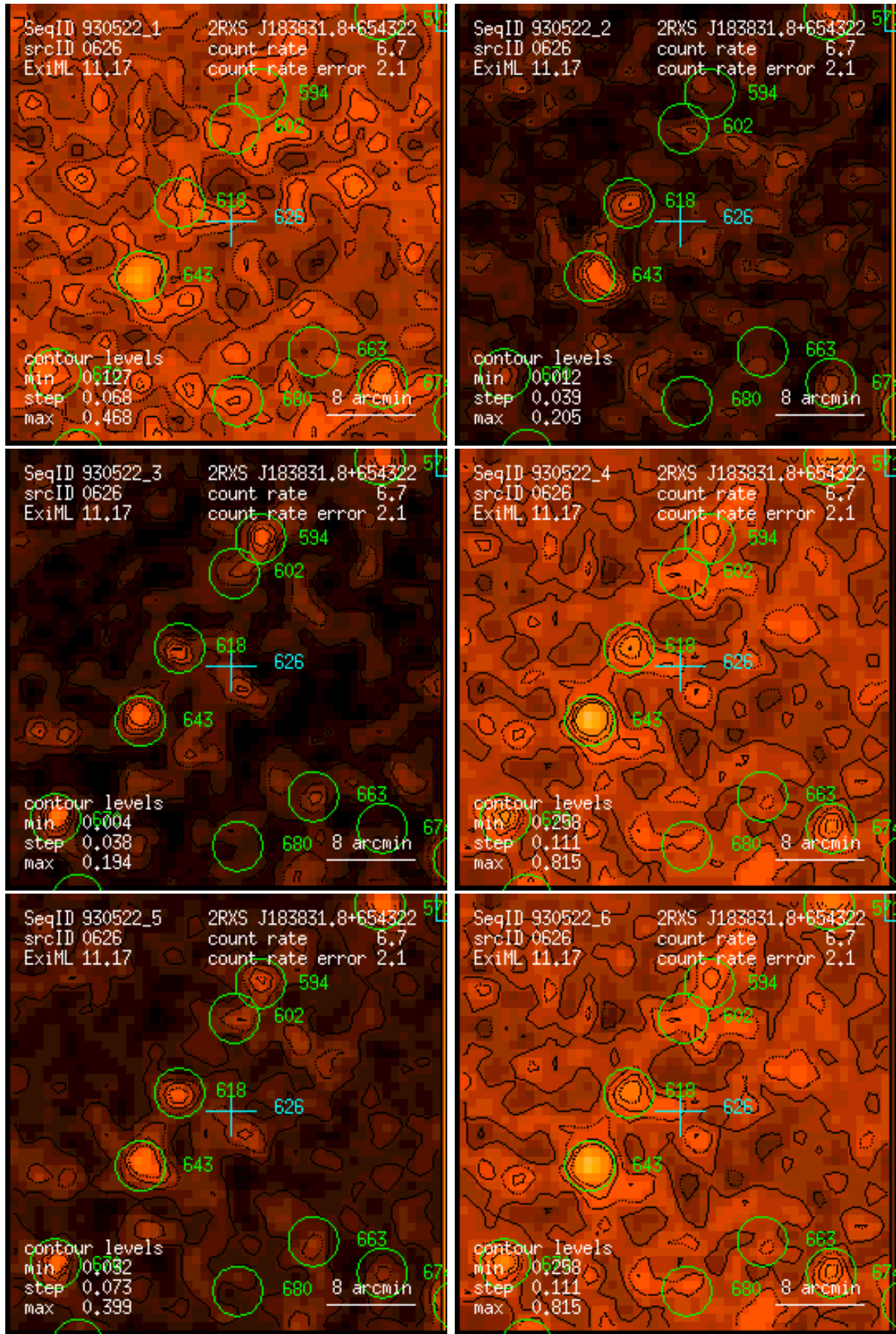
Figure 626: RASS 930522: detection 0626: band rate images, Gaussian filter: (1) PSPC channels 11 – 41, (2) 52 – 90, (3) 91 – 201, (4) 11 – 235, (5) 52 – 201, (6) 11 – 201. Broad band rates in counts/ks. Band rate contour levels in counts/ks/arcmin 2 .
