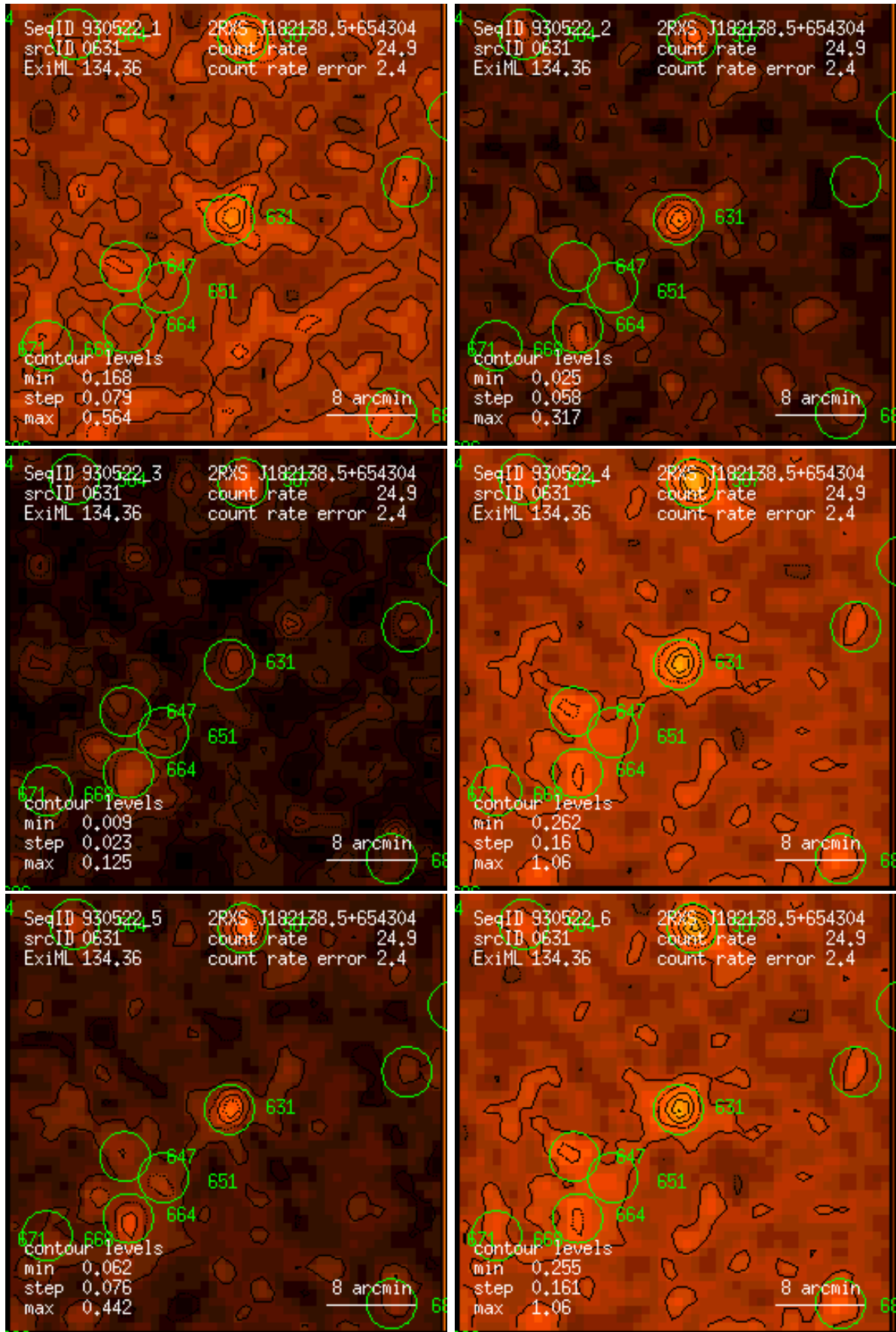
Figure 631: RASS 930522: detection 0631: band rate images, Gaussian filter: (1) PSPC channels 11 – 41, (2) 52 – 90, (3) 91 – 201, (4) 11 – 235, (5) 52 – 201, (6) 11 – 201. Broad band rates in counts/ks. Band rate contour levels in counts/ks/arcmin 2 .
