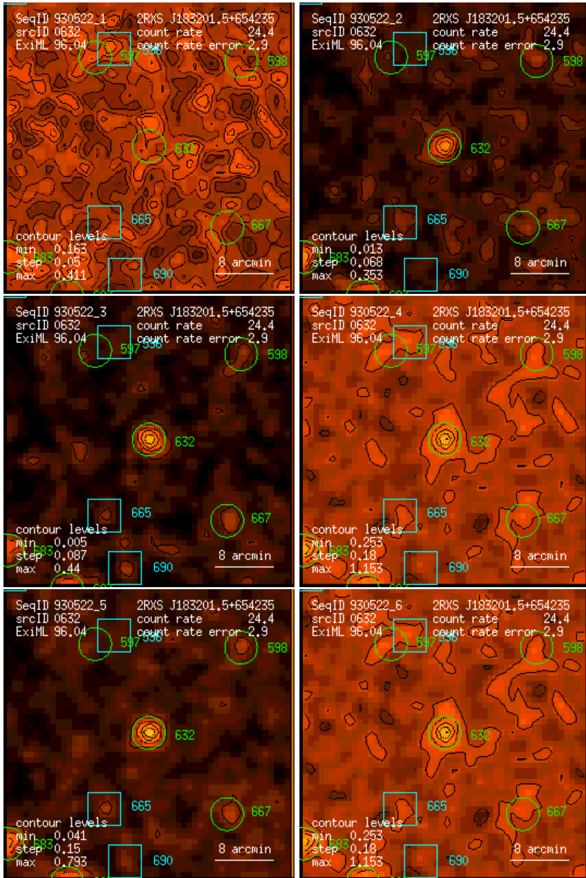
Figure 632: RASS 930522: detection 0632: band rate images, Gaussian filter: (1) PSPC channels 11 – 41, (2) 52 – 90, (3) 91 – 201, (4) 11 – 235, (5) 52 – 201, (6) 11 – 201. Broad band rates in counts/ks. Band rate contour levels in counts/ks/arcmin 2 .
