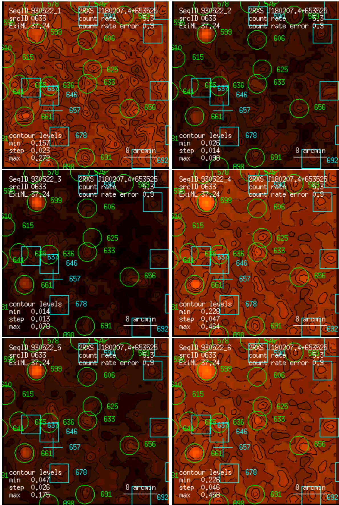
Figure 633: RASS 930522: detection 0633: band rate images, Gaussian filter: (1) PSPC channels 11 – 41, (2) 52 – 90, (3) 91 – 201, (4) 11 – 235, (5) 52 – 201, (6) 11 – 201. Broad band rates in counts/ks. Band rate contour levels in counts/ks/arcmin 2 .
