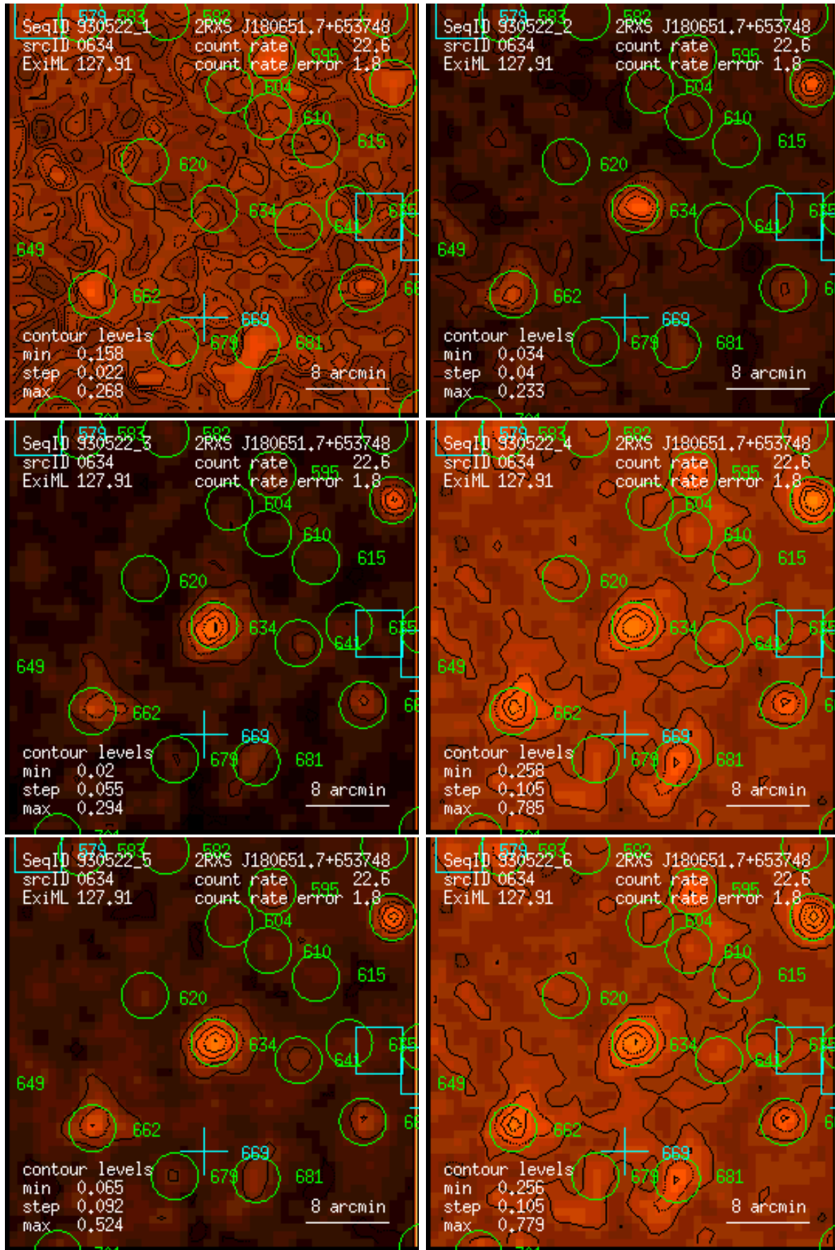
Figure 634: RASS 930522: detection 0634: band rate images, Gaussian filter: (1) PSPC channels 11 – 41, (2) 52 – 90, (3) 91 – 201, (4) 11 – 235, (5) 52 – 201, (6) 11 – 201. Broad band rates in counts/ks. Band rate contour levels in counts/ks/arcmin 2 .
