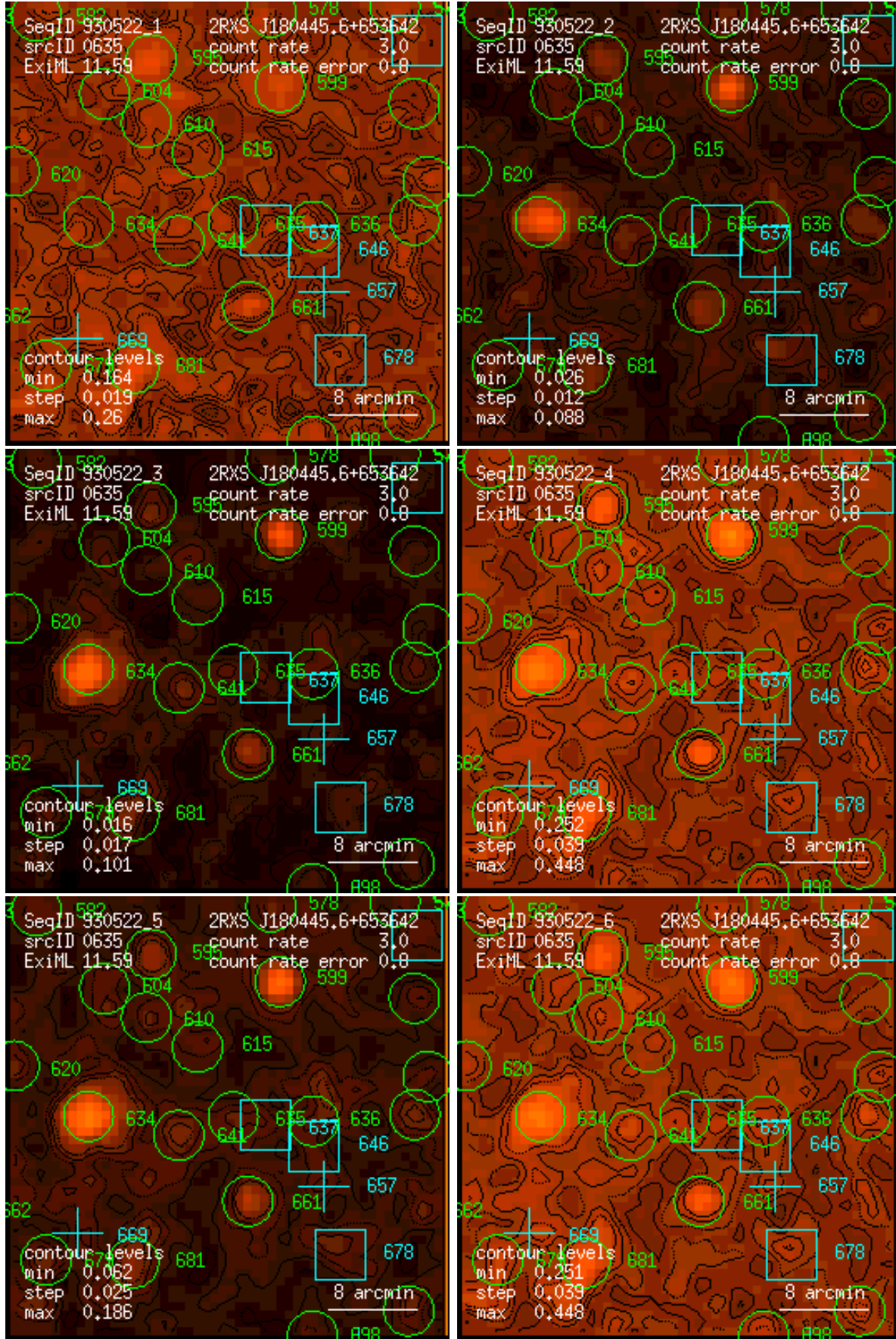
Figure 635: RASS 930522: detection 0635: band rate images, Gaussian filter: (1) PSPC channels 11 – 41, (2) 52 – 90, (3) 91 – 201, (4) 11 – 235, (5) 52 – 201, (6) 11 – 201. Broad band rates in counts/ks. Band rate contour levels in counts/ks/arcmin 2 .
