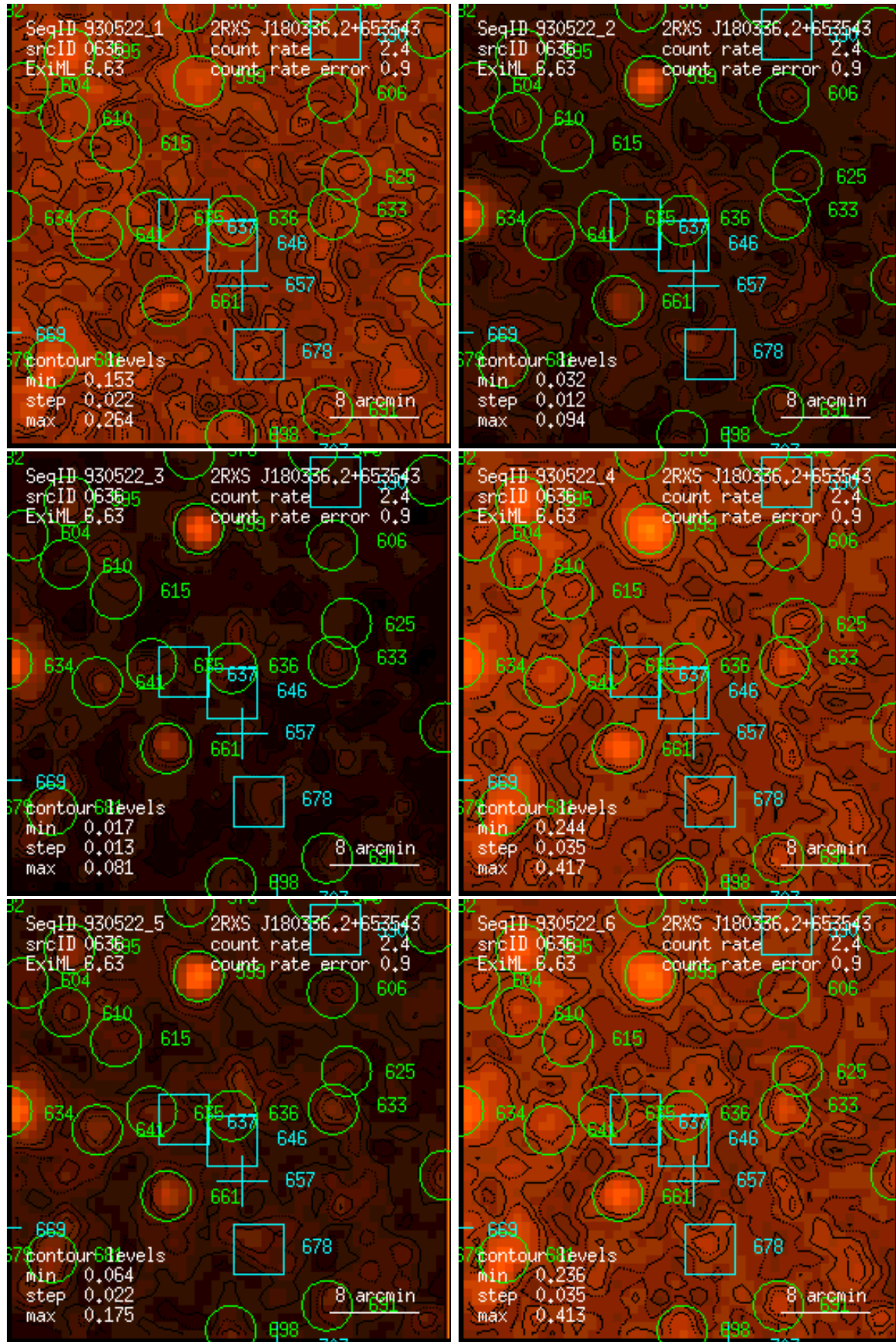
Figure 636: RASS 930522: detection 0636: band rate images, Gaussian filter: (1) PSPC channels 11 – 41, (2) 52 – 90, (3) 91 – 201, (4) 11 – 235, (5) 52 – 201, (6) 11 – 201. Broad band rates in counts/ks. Band rate contour levels in counts/ks/arcmin 2 .
