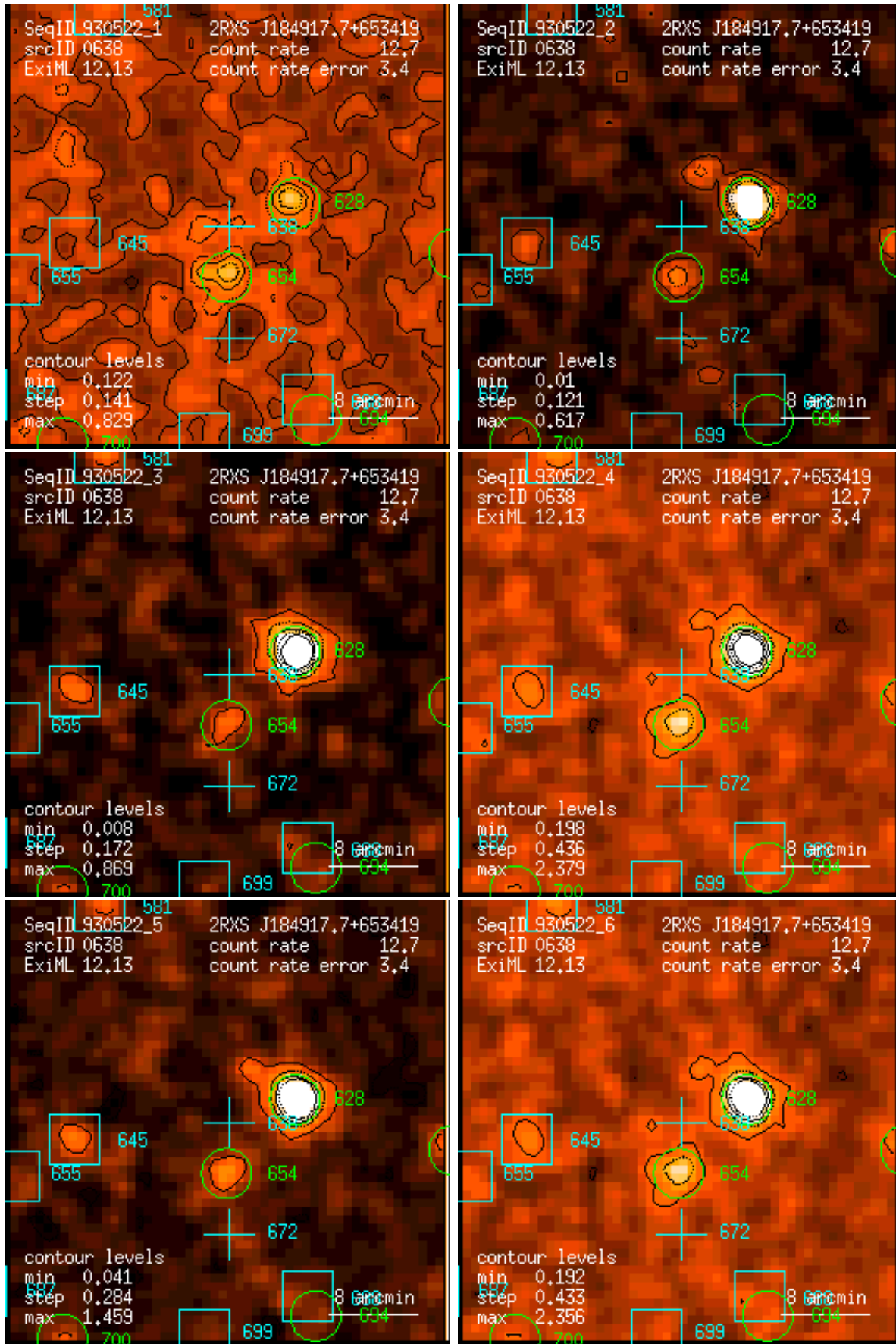
Figure 638: RASS 930522: detection 0638: band rate images, Gaussian filter: (1) PSPC channels 11 – 41, (2) 52 – 90, (3) 91 – 201, (4) 11 – 235, (5) 52 – 201, (6) 11 – 201. Broad band rates in counts/ks. Band rate contour levels in counts/ks/arcmin 2 .
