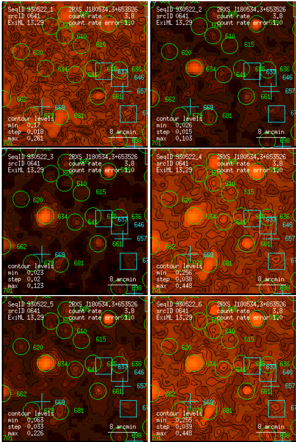
Figure 641: RASS 930522: detection 0641: band rate images, Gaussian filter: (1) PSPC channels 11 – 41, (2) 52 – 90, (3) 91 – 201, (4) 11 – 235, (5) 52 – 201, (6) 11 – 201. Broad band rates in counts/ks. Band rate contour levels in counts/ks/arcmin 2 .
