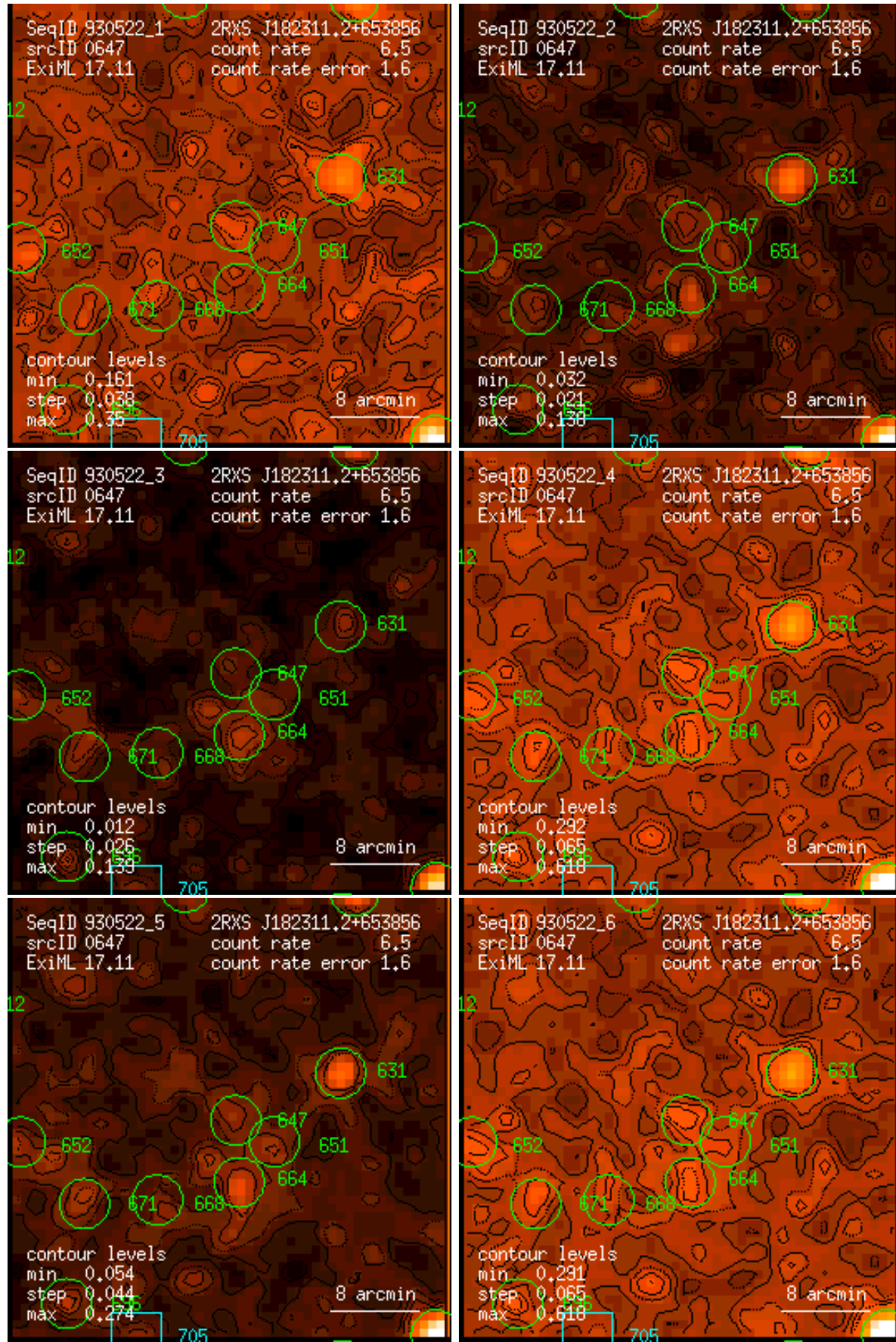
Figure 647: RASS 930522: detection 0647: band rate images, Gaussian filter: (1) PSPC channels 11 – 41, (2) 52 – 90, (3) 91 – 201, (4) 11 – 235, (5) 52 – 201, (6) 11 – 201. Broad band rates in counts/ks. Band rate contour levels in counts/ks/arcmin 2 .
