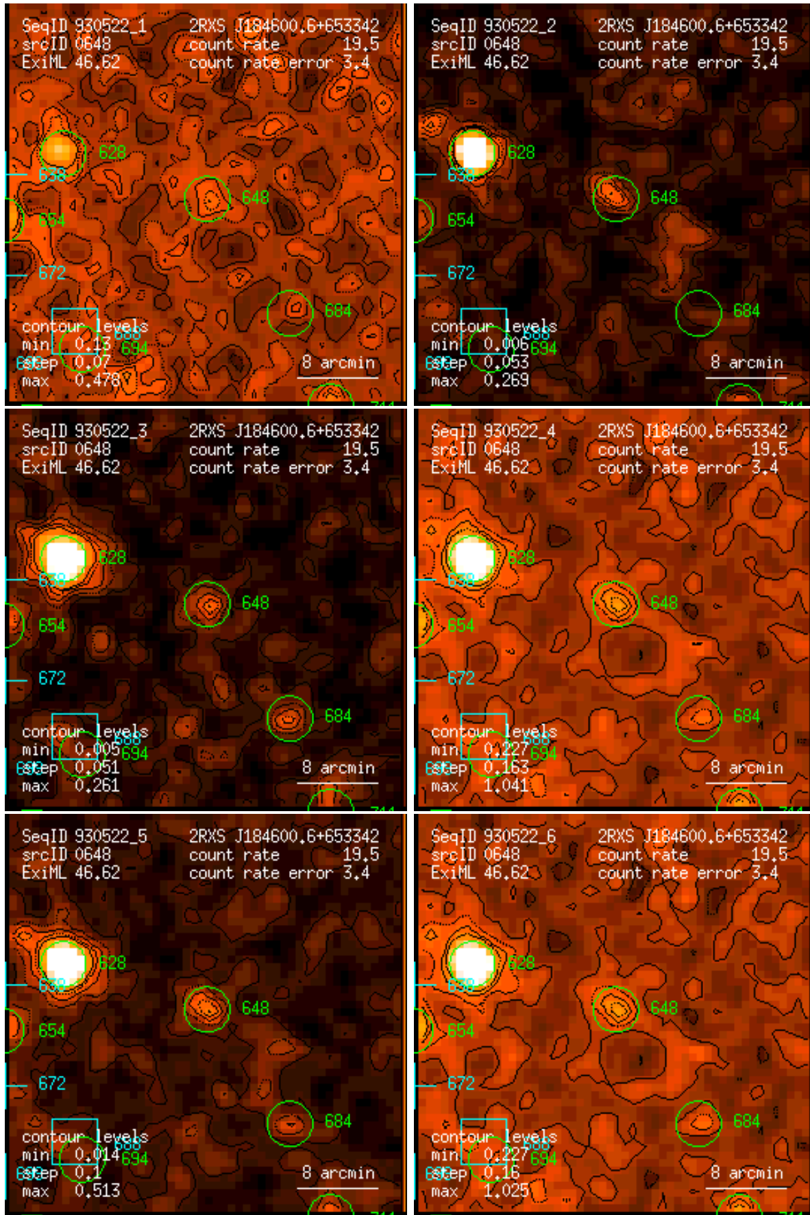
Figure 648: RASS 930522: detection 0648: band rate images, Gaussian filter: (1) PSPC channels 11 – 41, (2) 52 – 90, (3) 91 – 201, (4) 11 – 235, (5) 52 – 201, (6) 11 – 201. Broad band rates in counts/ks. Band rate contour levels in counts/ks/arcmin 2 .
