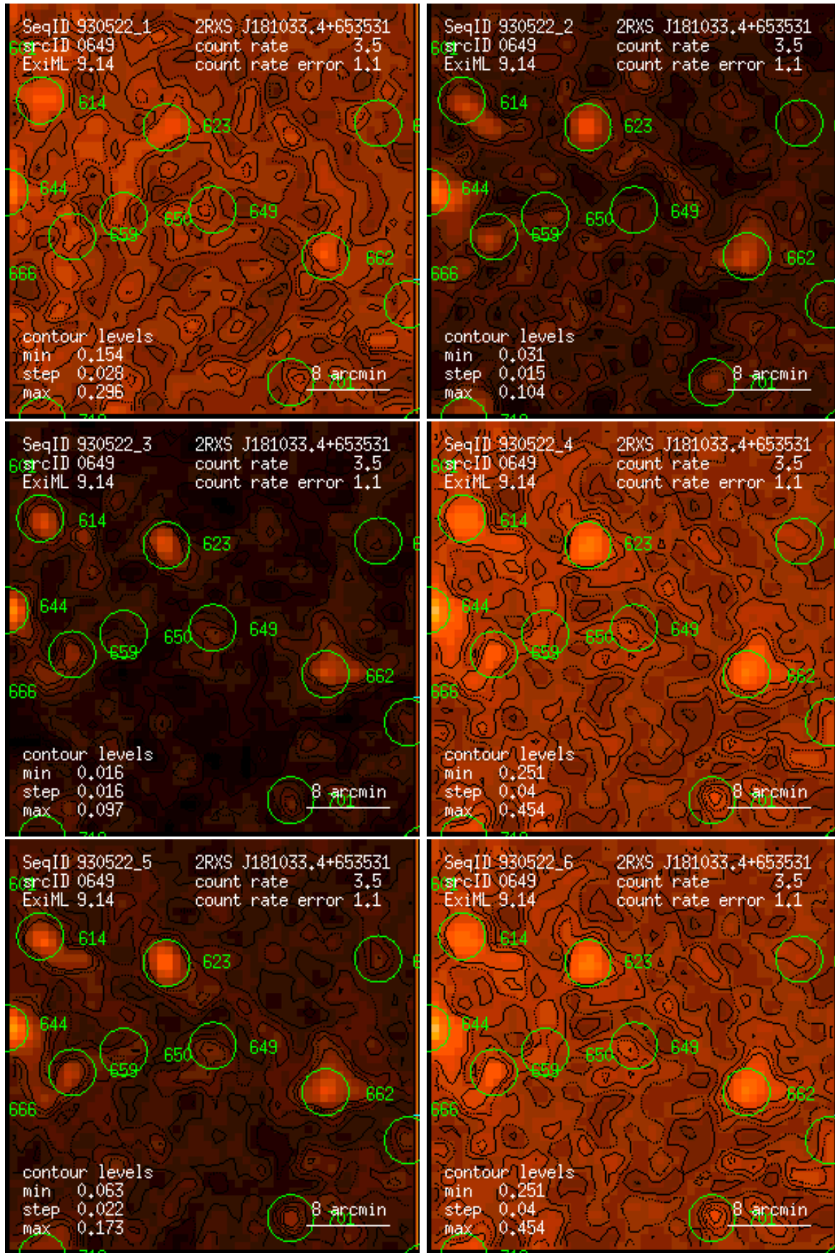
Figure 649: RASS 930522: detection 0649: band rate images, Gaussian filter: (1) PSPC channels 11 – 41, (2) 52 – 90, (3) 91 – 201, (4) 11 – 235, (5) 52 – 201, (6) 11 – 201. Broad band rates in counts/ks. Band rate contour levels in counts/ks/arcmin 2 .
