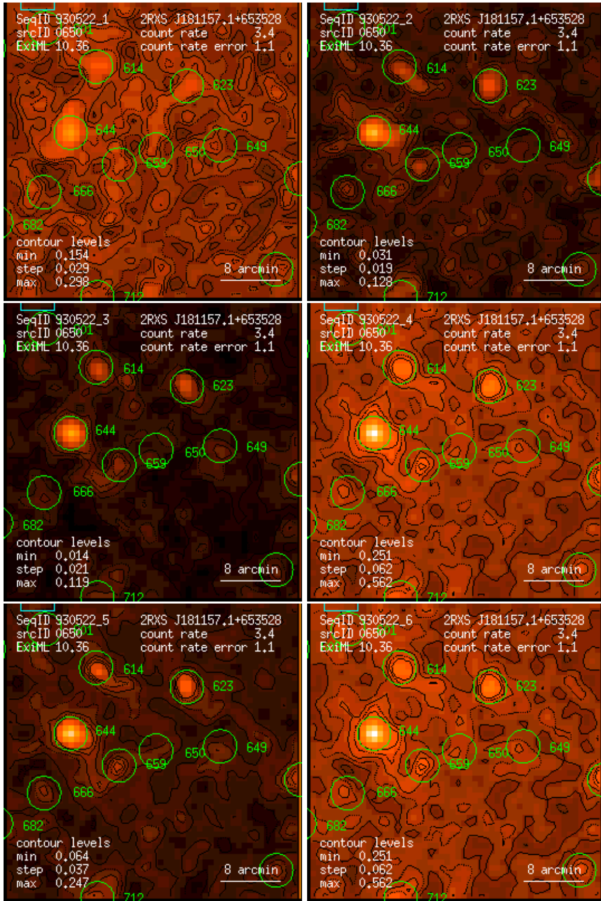
Figure 650: RASS 930522: detection 0650: band rate images, Gaussian filter: (1) PSPC channels 11 – 41, (2) 52 – 90, (3) 91 – 201, (4) 11 – 235, (5) 52 – 201, (6) 11 – 201. Broad band rates in counts/ks. Band rate contour levels in counts/ks/arcmin 2 .
