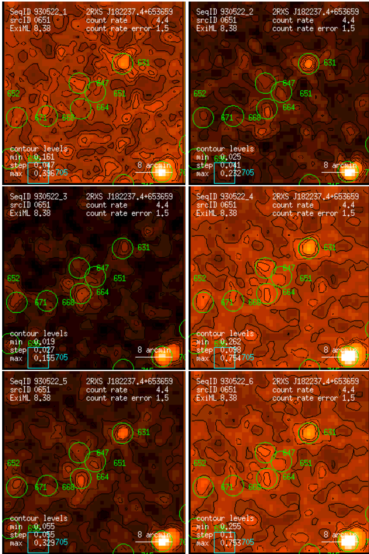
Figure 651: RASS 930522: detection 0651: band rate images, Gaussian filter: (1) PSPC channels 11 – 41, (2) 52 – 90, (3) 91 – 201, (4) 11 – 235, (5) 52 – 201, (6) 11 – 201. Broad band rates in counts/ks. Band rate contour levels in counts/ks/arcmin 2 .
