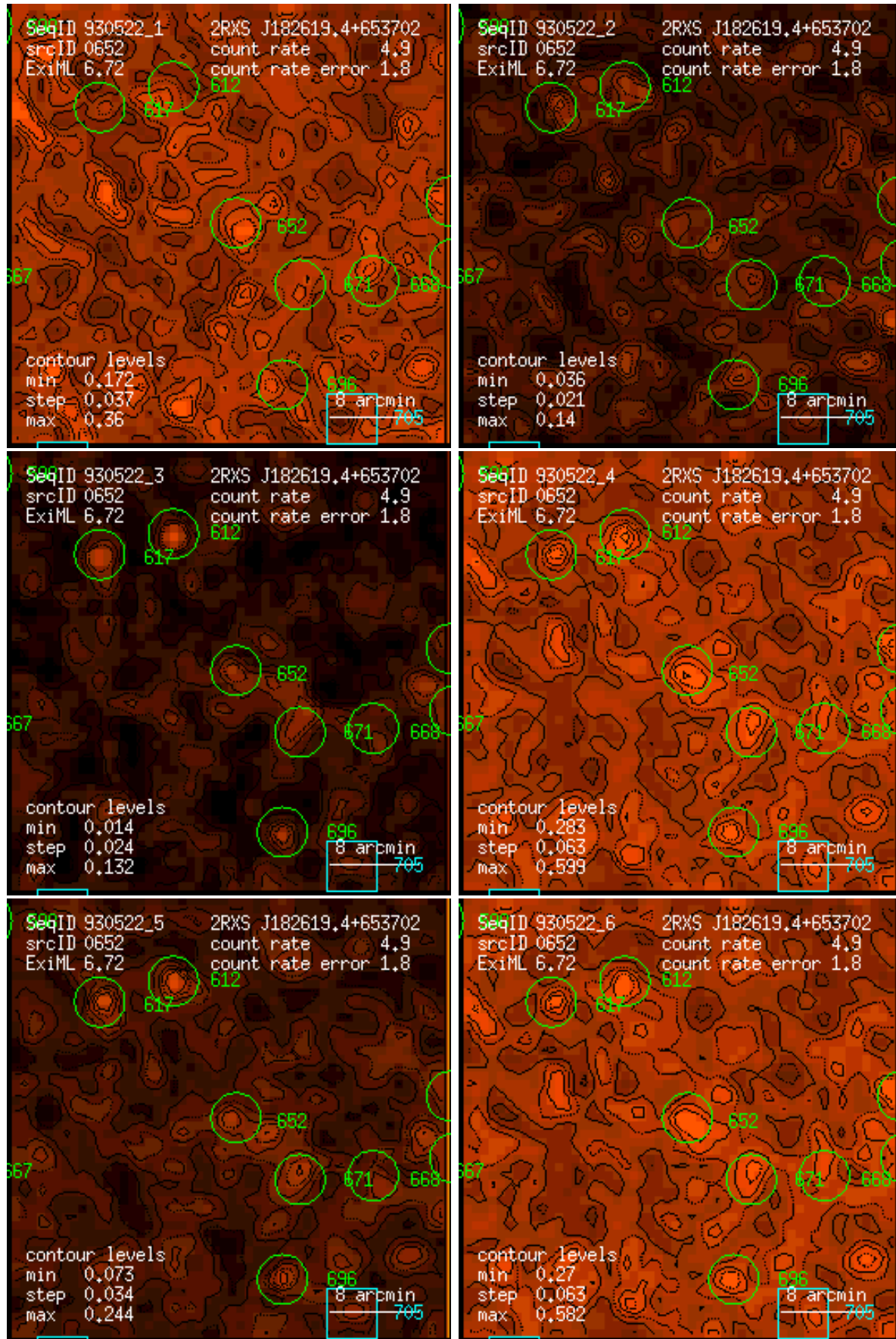
Figure 652: RASS 930522: detection 0652: band rate images, Gaussian filter: (1) PSPC channels 11 – 41, (2) 52 – 90, (3) 91 – 201, (4) 11 – 235, (5) 52 – 201, (6) 11 – 201. Broad band rates in counts/ks. Band rate contour levels in counts/ks/arcmin 2 .
